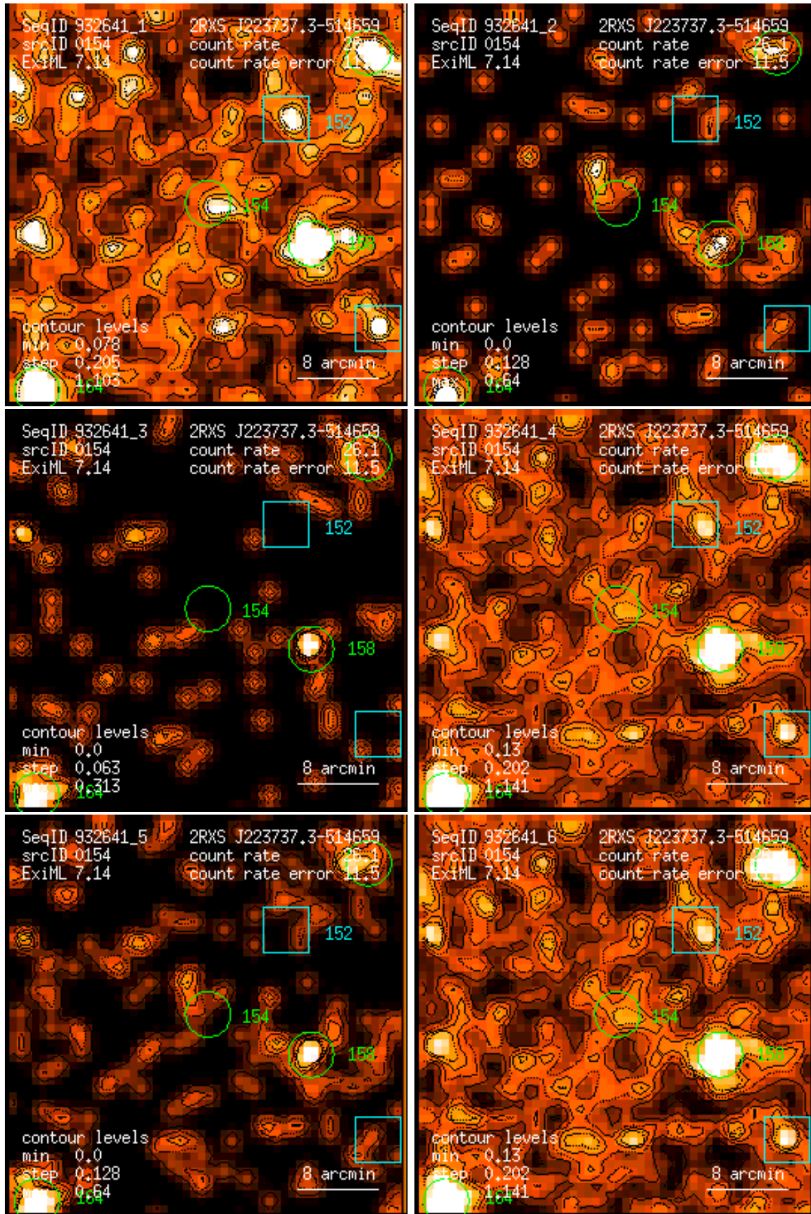
Figure 154: RASS 932641: detection 0154: band rate images, Gaussian filter: (1) PSPC channels 11 – 41, (2) 52 – 90, (3) 91 – 201, (4) 11 – 235, (5) 52 – 201, (6) 11 – 201. Broad band rates in counts/ks. Band rate contour levels in counts/ks/arcmin 2 .
