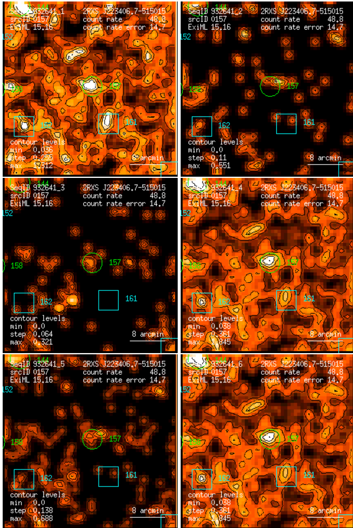
Figure 157: RASS 932641: detection 0157: band rate images, Gaussian filter: (1) PSPC channels 11 – 41, (2) 52 – 90, (3) 91 – 201, (4) 11 – 235, (5) 52 – 201, (6) 11 – 201. Broad band rates in counts/ks. Band rate contour levels in counts/ks/arcmin 2 .
