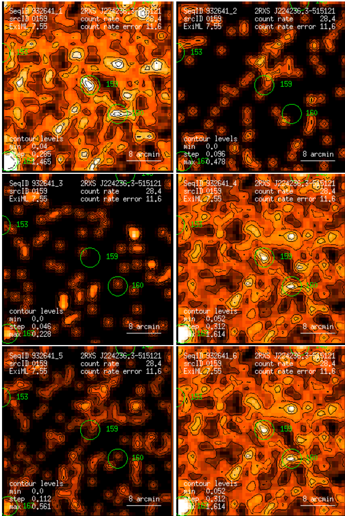
Figure 159: RASS 932641: detection 0159: band rate images, Gaussian filter: (1) PSPC channels 11 – 41, (2) 52 – 90, (3) 91 – 201, (4) 11 – 235, (5) 52 – 201, (6) 11 – 201. Broad band rates in counts/ks. Band rate contour levels in counts/ks/arcmin 2 .
