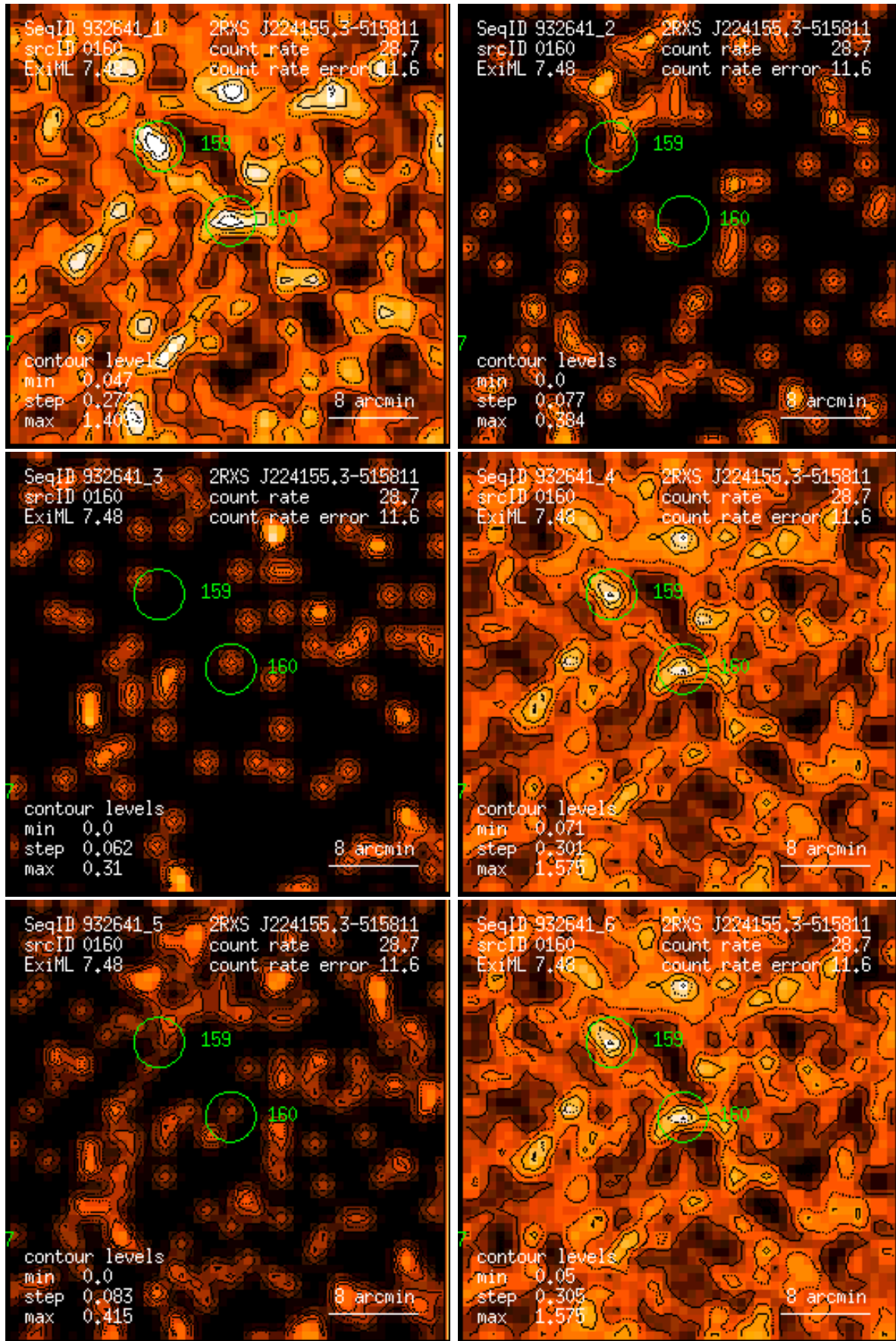
Figure 160: RASS 932641: detection 0160: band rate images, Gaussian filter: (1) PSPC channels 11 – 41, (2) 52 – 90, (3) 91 – 201, (4) 11 – 235, (5) 52 – 201, (6) 11 – 201. Broad band rates in counts/ks. Band rate contour levels in counts/ks/arcmin 2 .
