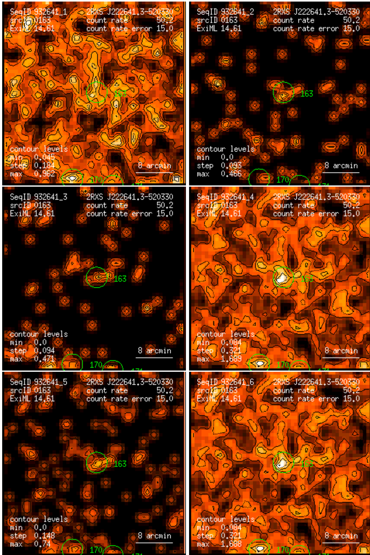
Figure 163: RASS 932641: detection 0163: band rate images, Gaussian filter: (1) PSPC channels 11 – 41, (2) 52 – 90, (3) 91 – 201, (4) 11 – 235, (5) 52 – 201, (6) 11 – 201. Broad band rates in counts/ks. Band rate contour levels in counts/ks/arcmin 2 .
