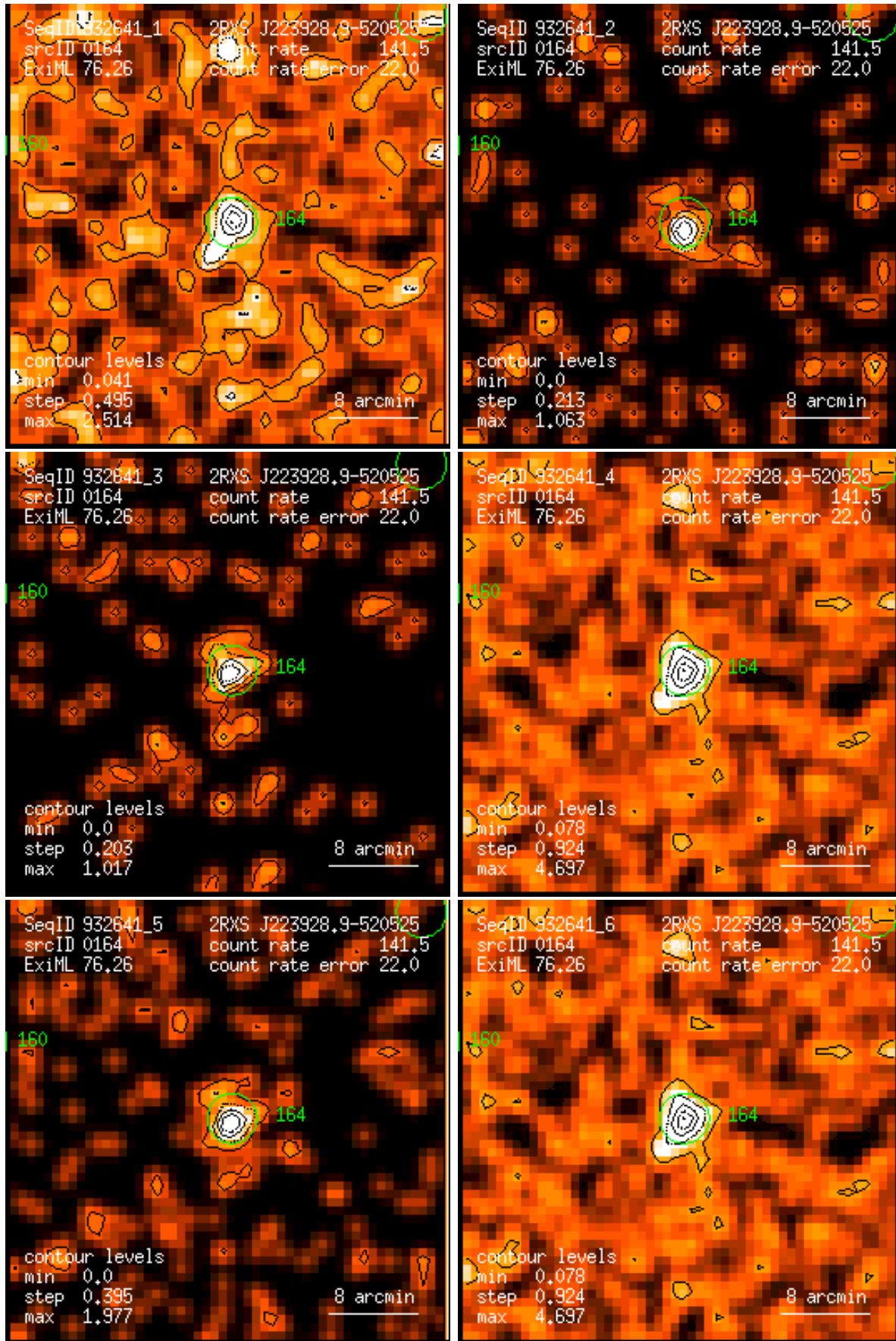
Figure 164: RASS 932641: detection 0164: band rate images, Gaussian filter: (1) PSPC channels 11 – 41, (2) 52 – 90, (3) 91 – 201, (4) 11 – 235, (5) 52 – 201, (6) 11 – 201. Broad band rates in counts/ks. Band rate contour levels in counts/ks/arcmin 2 .
