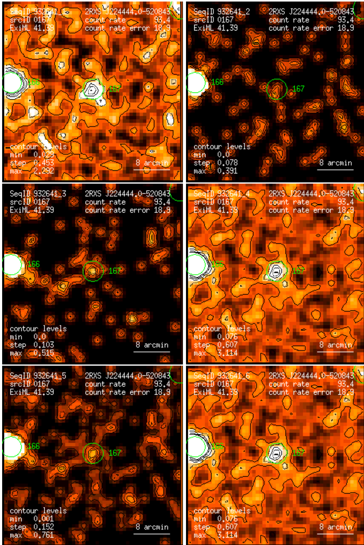
Figure 167: RASS 932641: detection 0167: band rate images, Gaussian filter: (1) PSPC channels 11 – 41, (2) 52 – 90, (3) 91 – 201, (4) 11 – 235, (5) 52 – 201, (6) 11 – 201. Broad band rates in counts/ks. Band rate contour levels in counts/ks/arcmin 2 .
