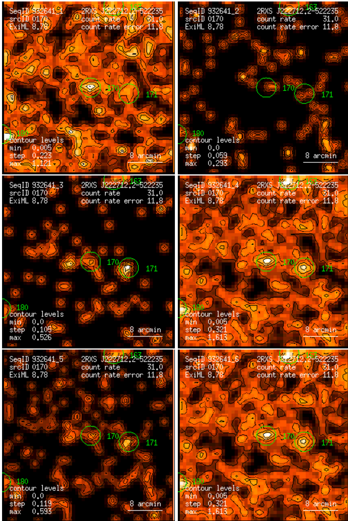
Figure 170: RASS 932641: detection 0170: band rate images, Gaussian filter: (1) PSPC channels 11 – 41, (2) 52 – 90, (3) 91 – 201, (4) 11 – 235, (5) 52 – 201, (6) 11 – 201. Broad band rates in counts/ks. Band rate contour levels in counts/ks/arcmin 2 .
