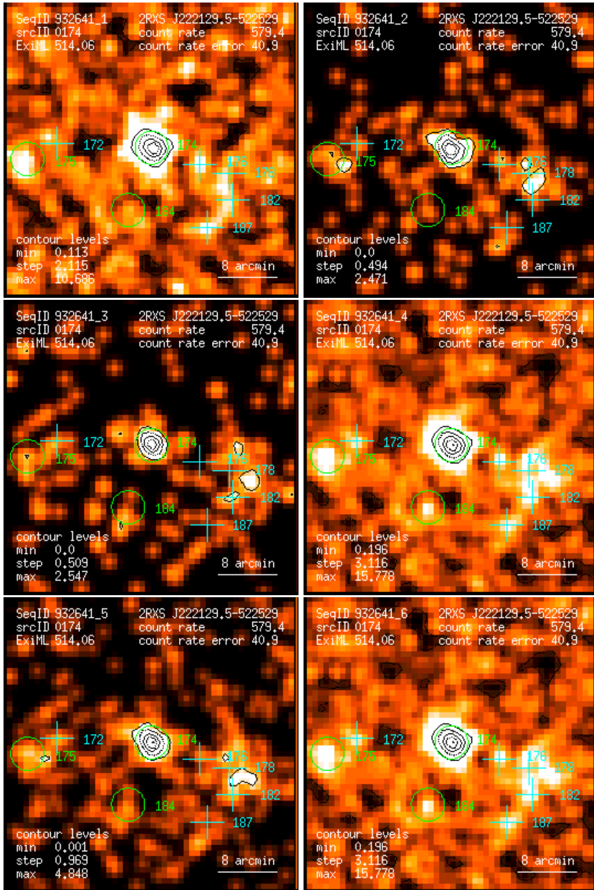
Figure 174: RASS 932641: detection 0174: band rate images, Gaussian filter: (1) PSPC channels 11 – 41, (2) 52 – 90, (3) 91 – 201, (4) 11 – 235, (5) 52 – 201, (6) 11 – 201. Broad band rates in counts/ks. Band rate contour levels in counts/ks/arcmin 2 .
