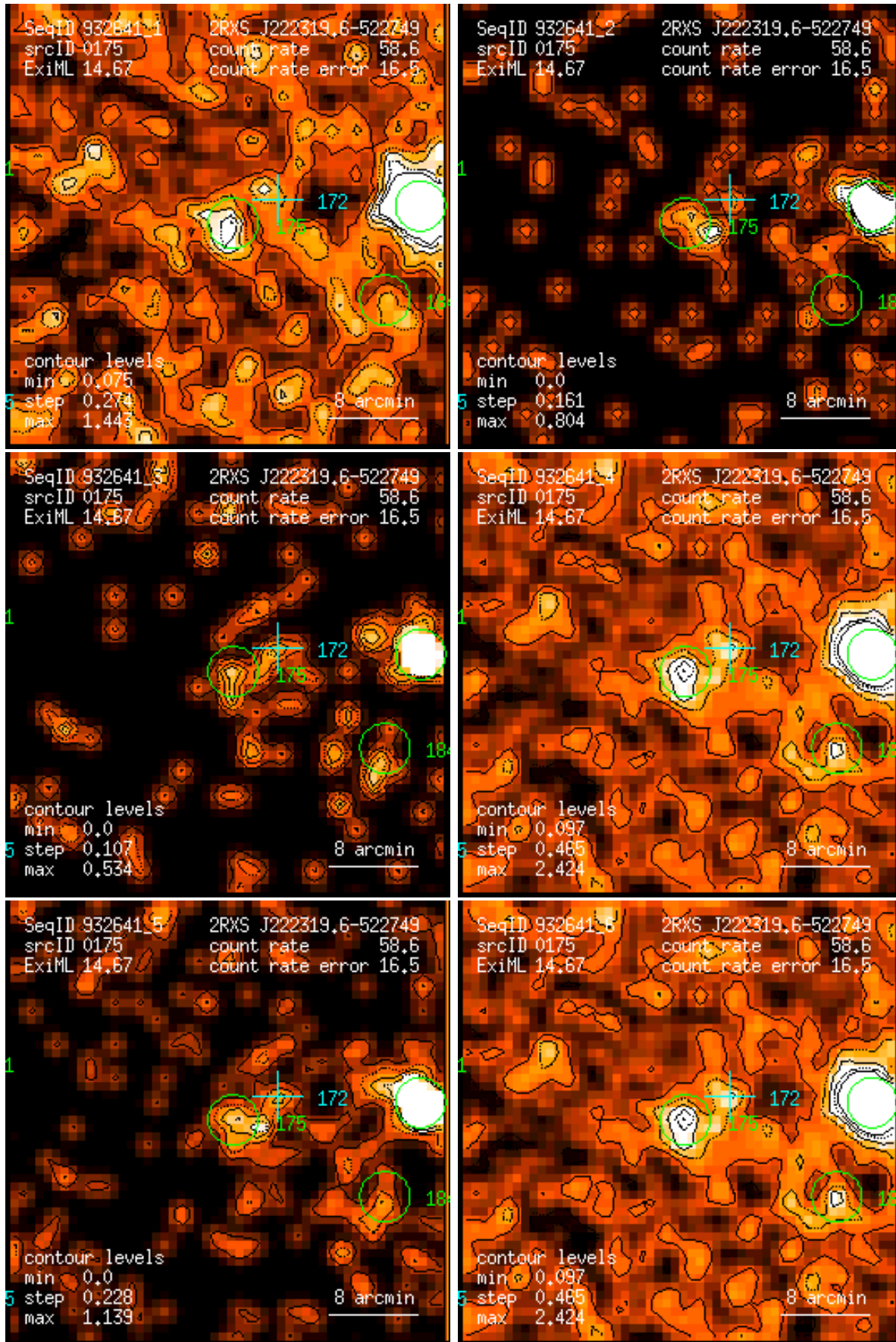
Figure 175: RASS 932641: detection 0175: band rate images, Gaussian filter: (1) PSPC channels 11 – 41, (2) 52 – 90, (3) 91 – 201, (4) 11 – 235, (5) 52 – 201, (6) 11 – 201. Broad band rates in counts/ks. Band rate contour levels in counts/ks/arcmin 2 .
