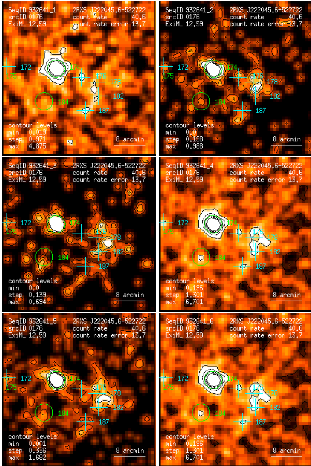
Figure 176: RASS 932641: detection 0176: band rate images, Gaussian filter: (1) PSPC channels 11 – 41, (2) 52 – 90, (3) 91 – 201, (4) 11 – 235, (5) 52 – 201, (6) 11 – 201. Broad band rates in counts/ks. Band rate contour levels in counts/ks/arcmin 2 .
