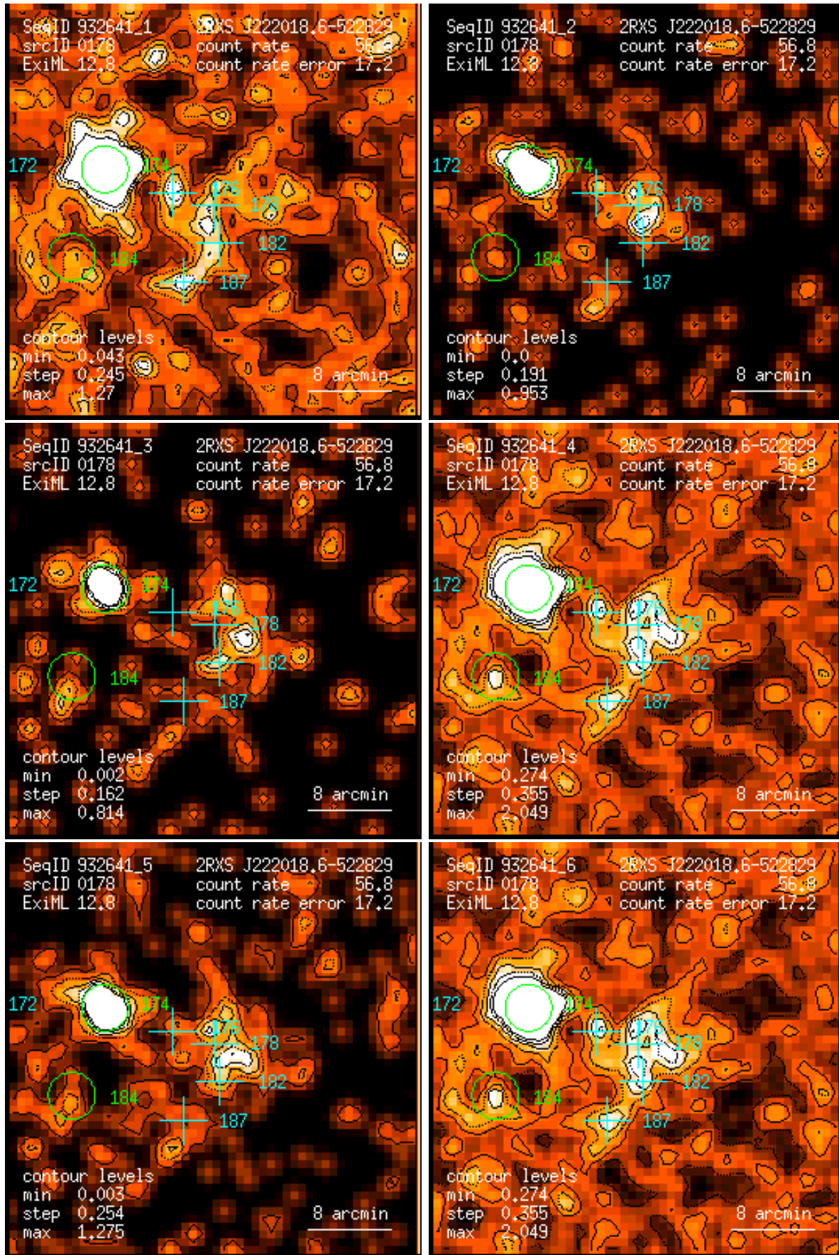
Figure 178: RASS 932641: detection 0178: band rate images, Gaussian filter: (1) PSPC channels 11 – 41, (2) 52 – 90, (3) 91 – 201, (4) 11 – 235, (5) 52 – 201, (6) 11 – 201. Broad band rates in counts/ks. Band rate contour levels in counts/ks/arcmin 2 .
