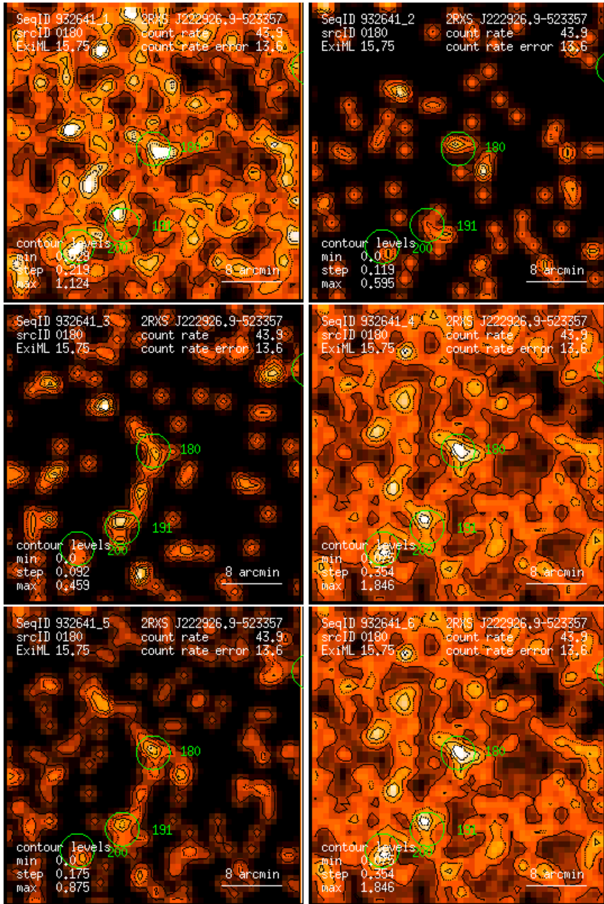
Figure 180: RASS 932641: detection 0180: band rate images, Gaussian filter: (1) PSPC channels 11 – 41, (2) 52 – 90, (3) 91 – 201, (4) 11 – 235, (5) 52 – 201, (6) 11 – 201. Broad band rates in counts/ks. Band rate contour levels in counts/ks/arcmin 2 .
