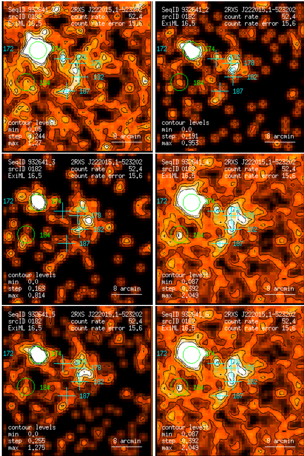
Figure 182: RASS 932641: detection 0182: band rate images, Gaussian filter: (1) PSPC channels 11 – 41, (2) 52 – 90, (3) 91 – 201, (4) 11 – 235, (5) 52 – 201, (6) 11 – 201. Broad band rates in counts/ks. Band rate contour levels in counts/ks/arcmin 2 .
