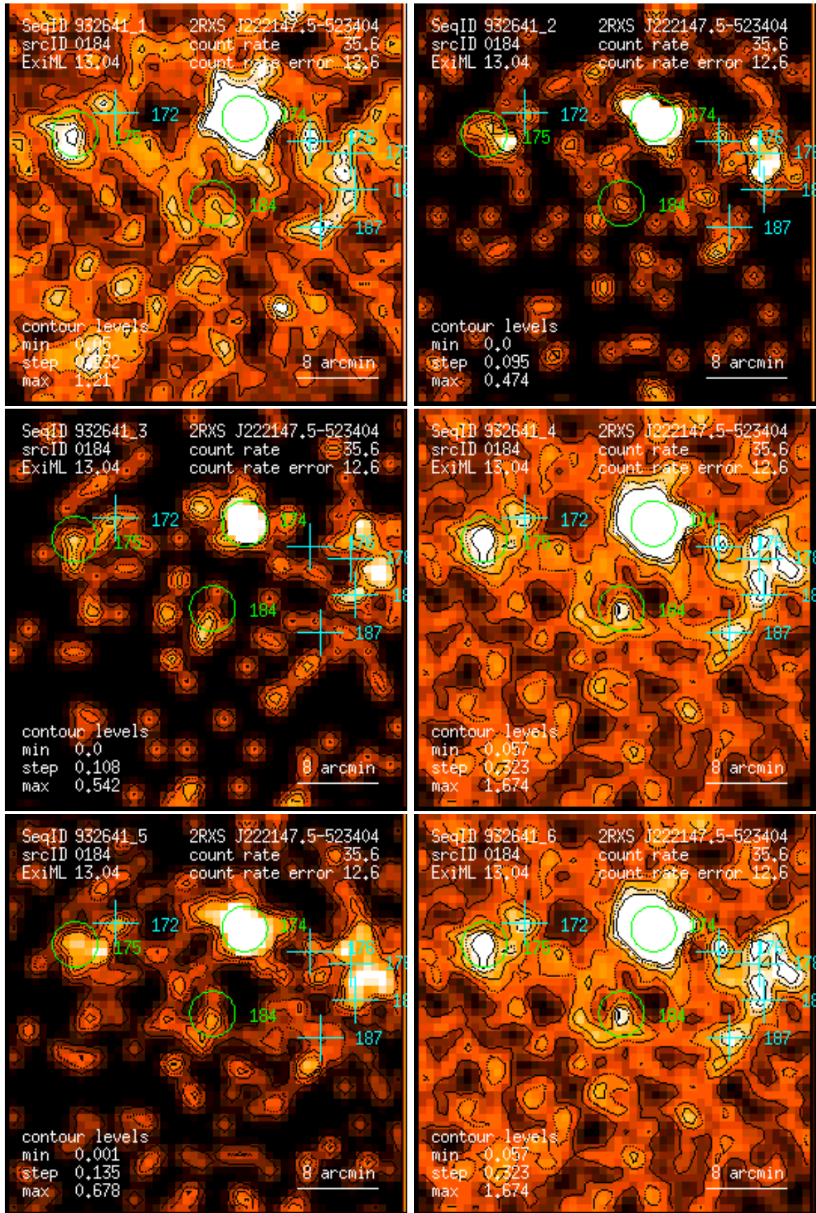
Figure 184: RASS 932641: detection 0184: band rate images, Gaussian filter: (1) PSPC channels 11 – 41, (2) 52 – 90, (3) 91 – 201, (4) 11 – 235, (5) 52 – 201, (6) 11 – 201. Broad band rates in counts/ks. Band rate contour levels in counts/ks/arcmin 2 .
