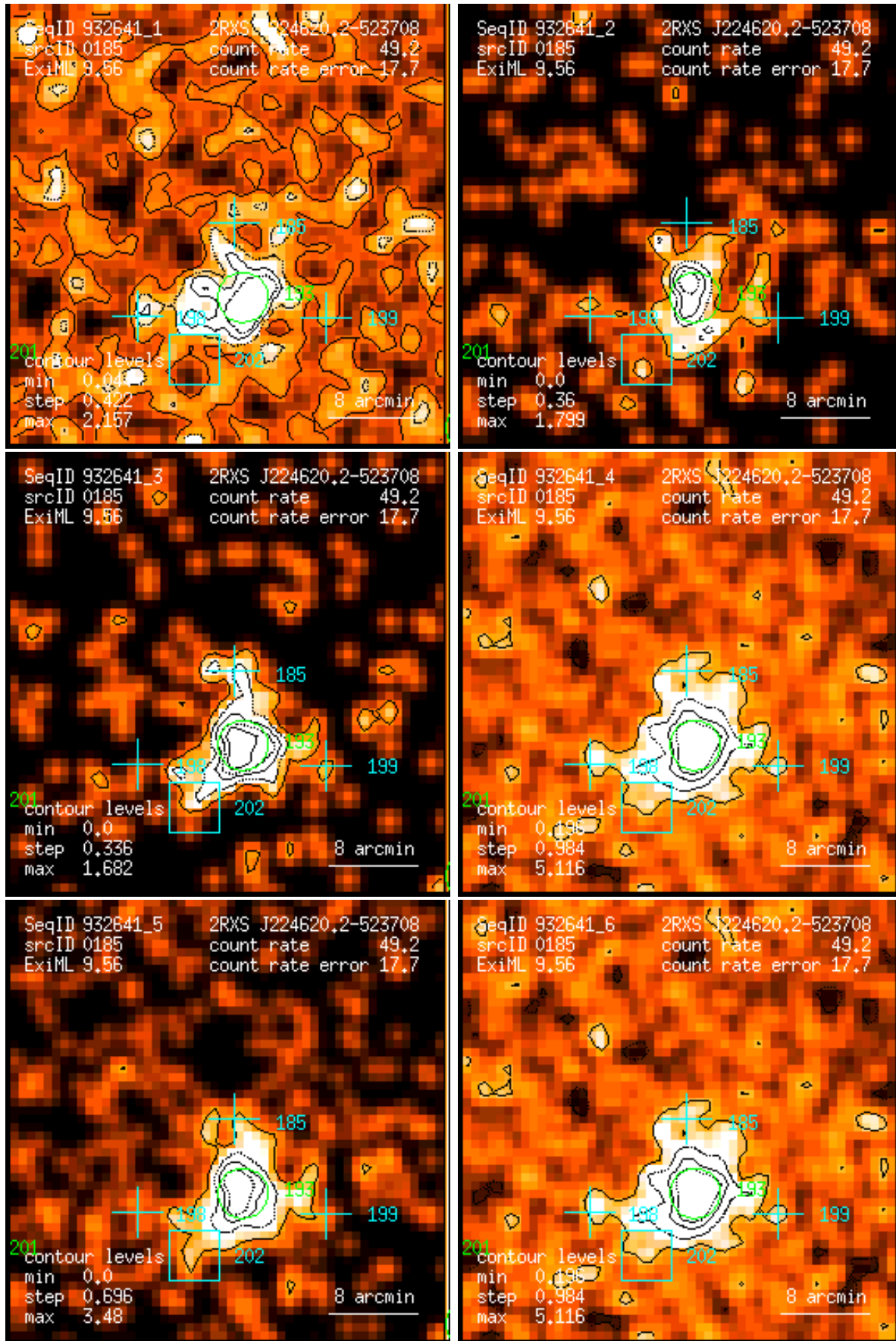
Figure 185: RASS 932641: detection 0185: band rate images, Gaussian filter: (1) PSPC channels 11 – 41, (2) 52 – 90, (3) 91 – 201, (4) 11 – 235, (5) 52 – 201, (6) 11 – 201. Broad band rates in counts/ks. Band rate contour levels in counts/ks/arcmin 2 .
