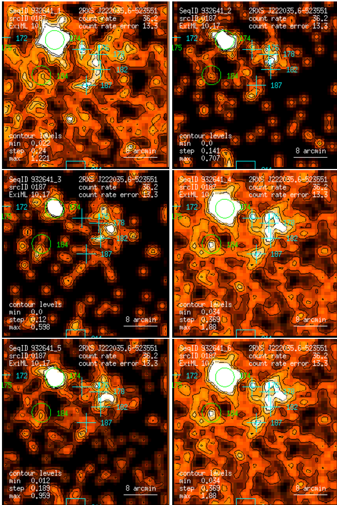
Figure 187: RASS 932641: detection 0187: band rate images, Gaussian filter: (1) PSPC channels 11 – 41, (2) 52 – 90, (3) 91 – 201, (4) 11 – 235, (5) 52 – 201, (6) 11 – 201. Broad band rates in counts/ks. Band rate contour levels in counts/ks/arcmin 2 .
