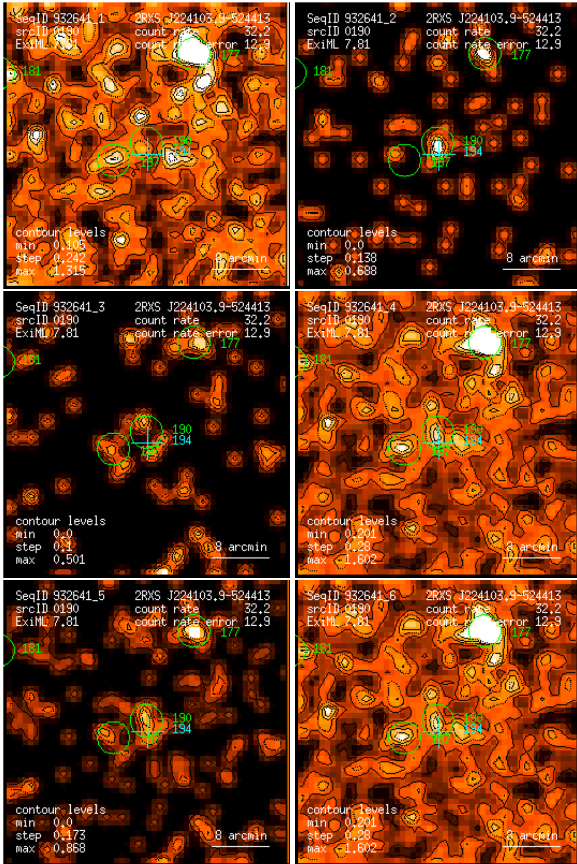
Figure 190: RASS 932641: detection 0190: band rate images, Gaussian filter: (1) PSPC channels 11 – 41, (2) 52 – 90, (3) 91 – 201, (4) 11 – 235, (5) 52 – 201, (6) 11 – 201. Broad band rates in counts/ks. Band rate contour levels in counts/ks/arcmin 2 .
