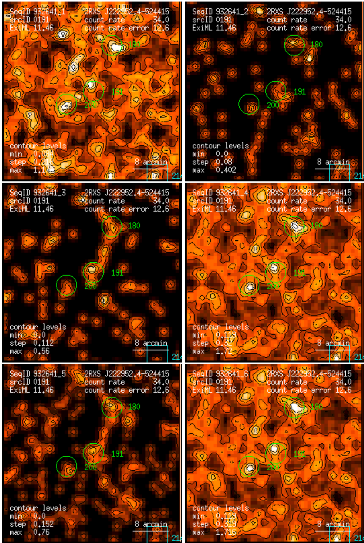
Figure 191: RASS 932641: detection 0191: band rate images, Gaussian filter: (1) PSPC channels 11 – 41, (2) 52 – 90, (3) 91 – 201, (4) 11 – 235, (5) 52 – 201, (6) 11 – 201. Broad band rates in counts/ks. Band rate contour levels in counts/ks/arcmin 2 .
