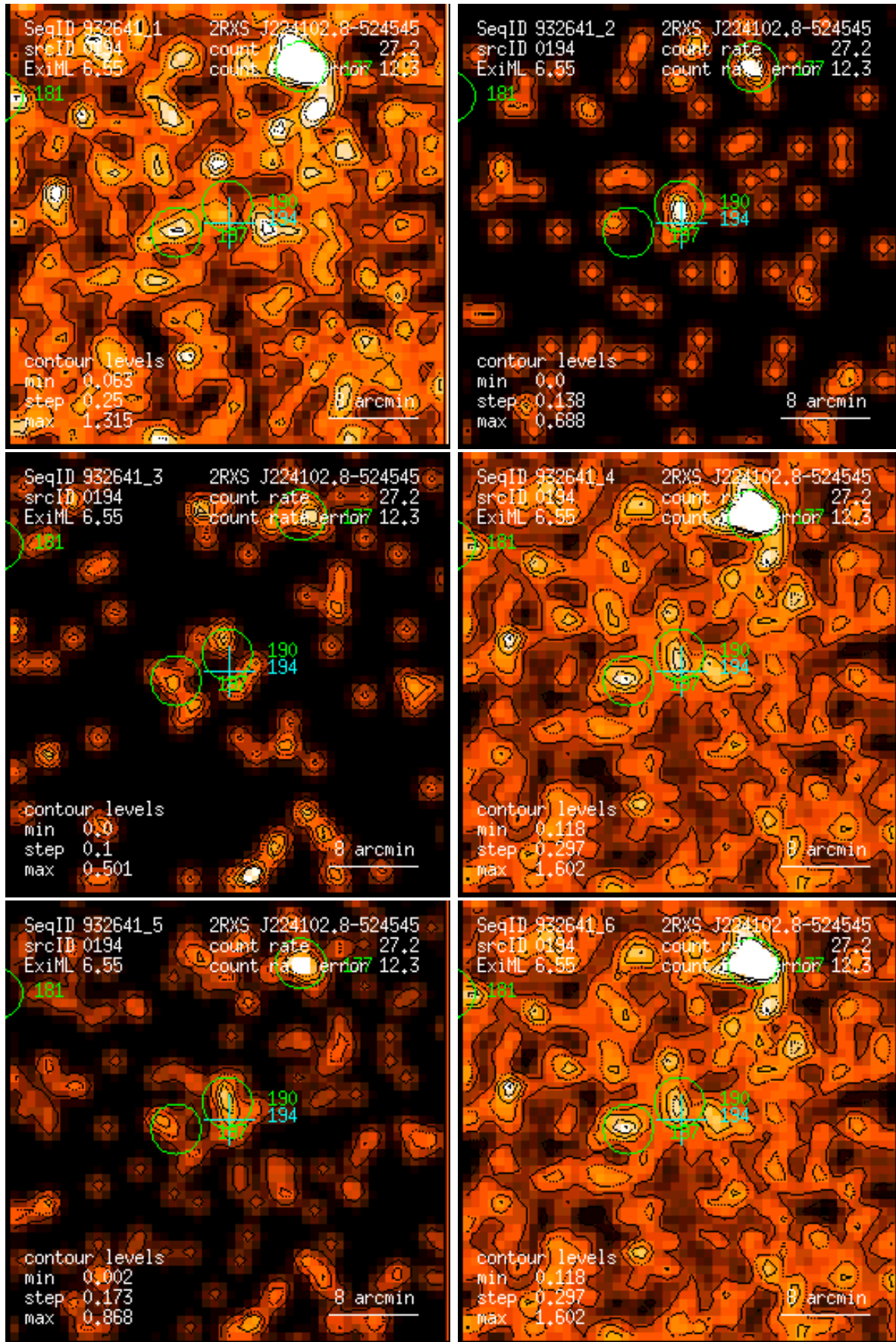
Figure 194: RASS 932641: detection 0194: band rate images, Gaussian filter: (1) PSPC channels 11 – 41, (2) 52 – 90, (3) 91 – 201, (4) 11 – 235, (5) 52 – 201, (6) 11 – 201. Broad band rates in counts/ks. Band rate contour levels in counts/ks/arcmin 2 .
