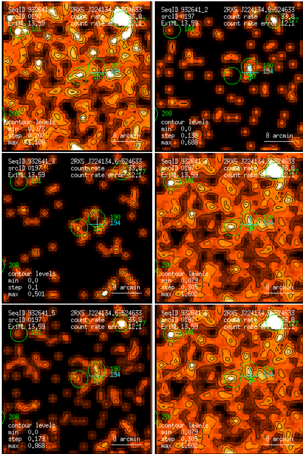
Figure 197: RASS 932641: detection 0197: band rate images, Gaussian filter: (1) PSPC channels 11 – 41, (2) 52 – 90, (3) 91 – 201, (4) 11 – 235, (5) 52 – 201, (6) 11 – 201. Broad band rates in counts/ks. Band rate contour levels in counts/ks/arcmin 2 .
