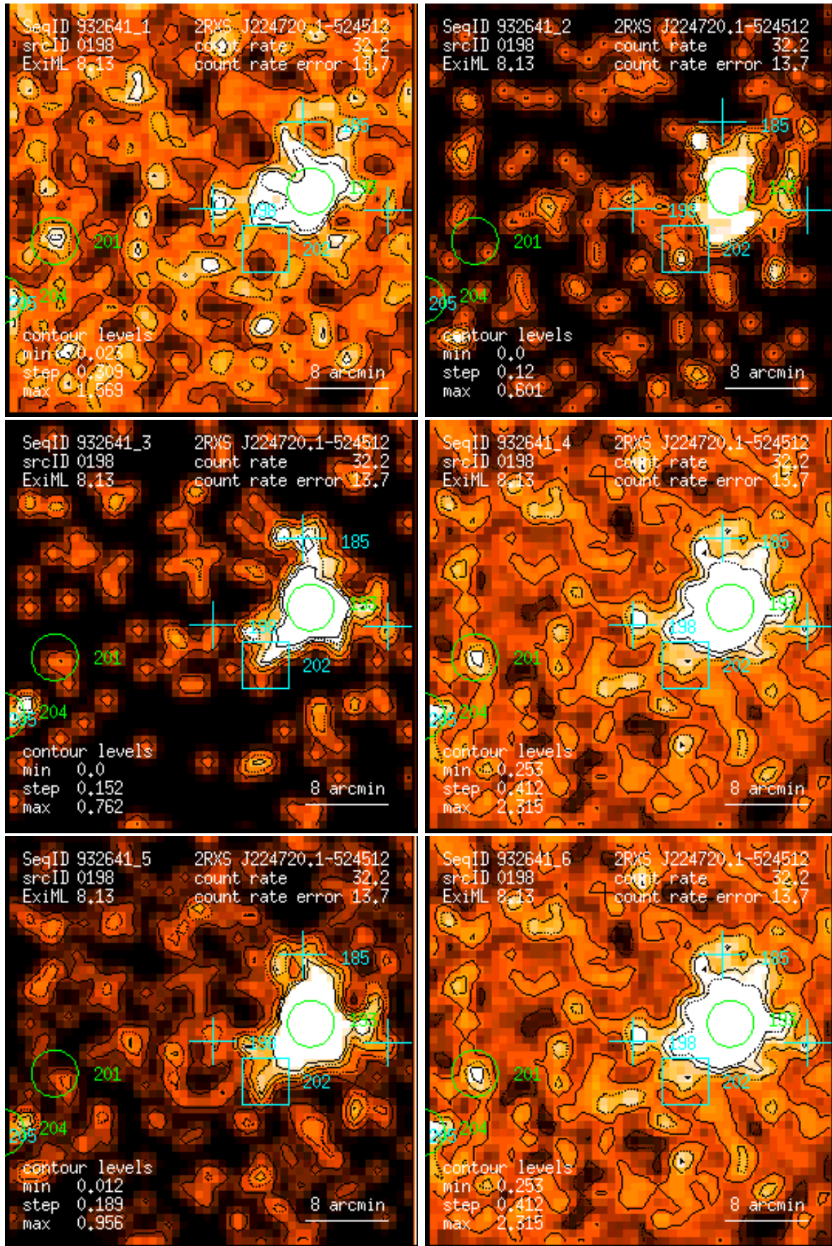
Figure 198: RASS 932641: detection 0198: band rate images, Gaussian filter: (1) PSPC channels 11 – 41, (2) 52 – 90, (3) 91 – 201, (4) 11 – 235, (5) 52 – 201, (6) 11 – 201. Broad band rates in counts/ks. Band rate contour levels in counts/ks/arcmin 2 .
