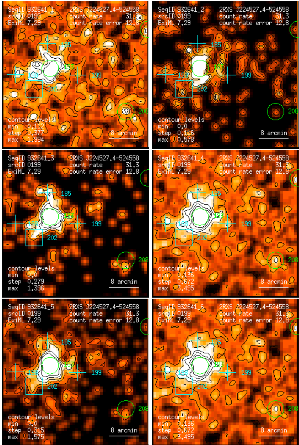
Figure 199: RASS 932641: detection 0199: band rate images, Gaussian filter: (1) PSPC channels 11 – 41, (2) 52 – 90, (3) 91 – 201, (4) 11 – 235, (5) 52 – 201, (6) 11 – 201. Broad band rates in counts/ks. Band rate contour levels in counts/ks/arcmin 2 .
