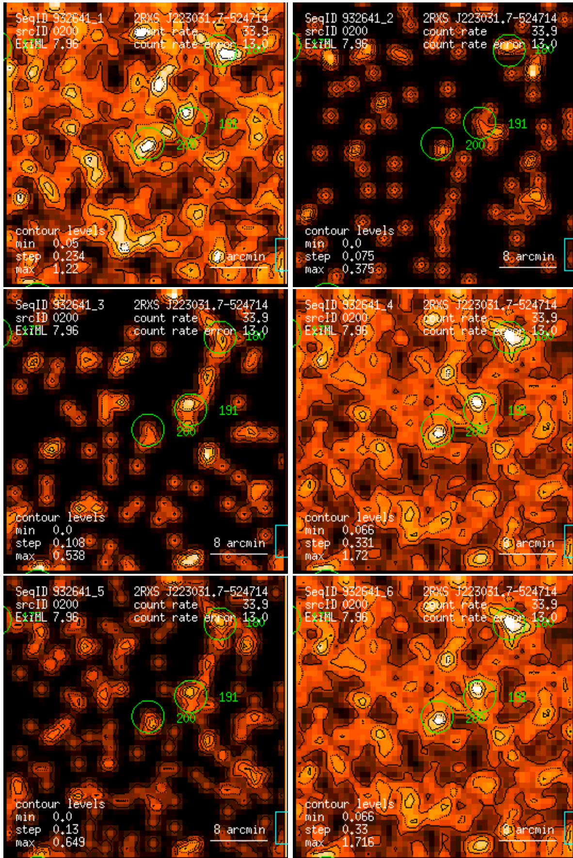
Figure 200: RASS 932641: detection 0200: band rate images, Gaussian filter: (1) PSPC channels 11 – 41, (2) 52 – 90, (3) 91 – 201, (4) 11 – 235, (5) 52 – 201, (6) 11 – 201. Broad band rates in counts/ks. Band rate contour levels in counts/ks/arcmin 2 .
