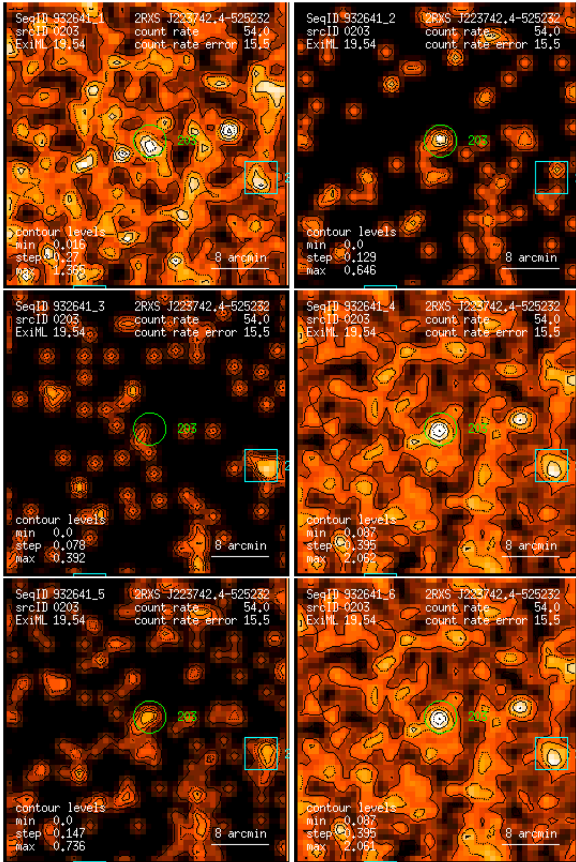
Figure 203: RASS 932641: detection 0203: band rate images, Gaussian filter: (1) PSPC channels 11 – 41, (2) 52 – 90, (3) 91 – 201, (4) 11 – 235, (5) 52 – 201, (6) 11 – 201. Broad band rates in counts/ks. Band rate contour levels in counts/ks/arcmin 2 .
