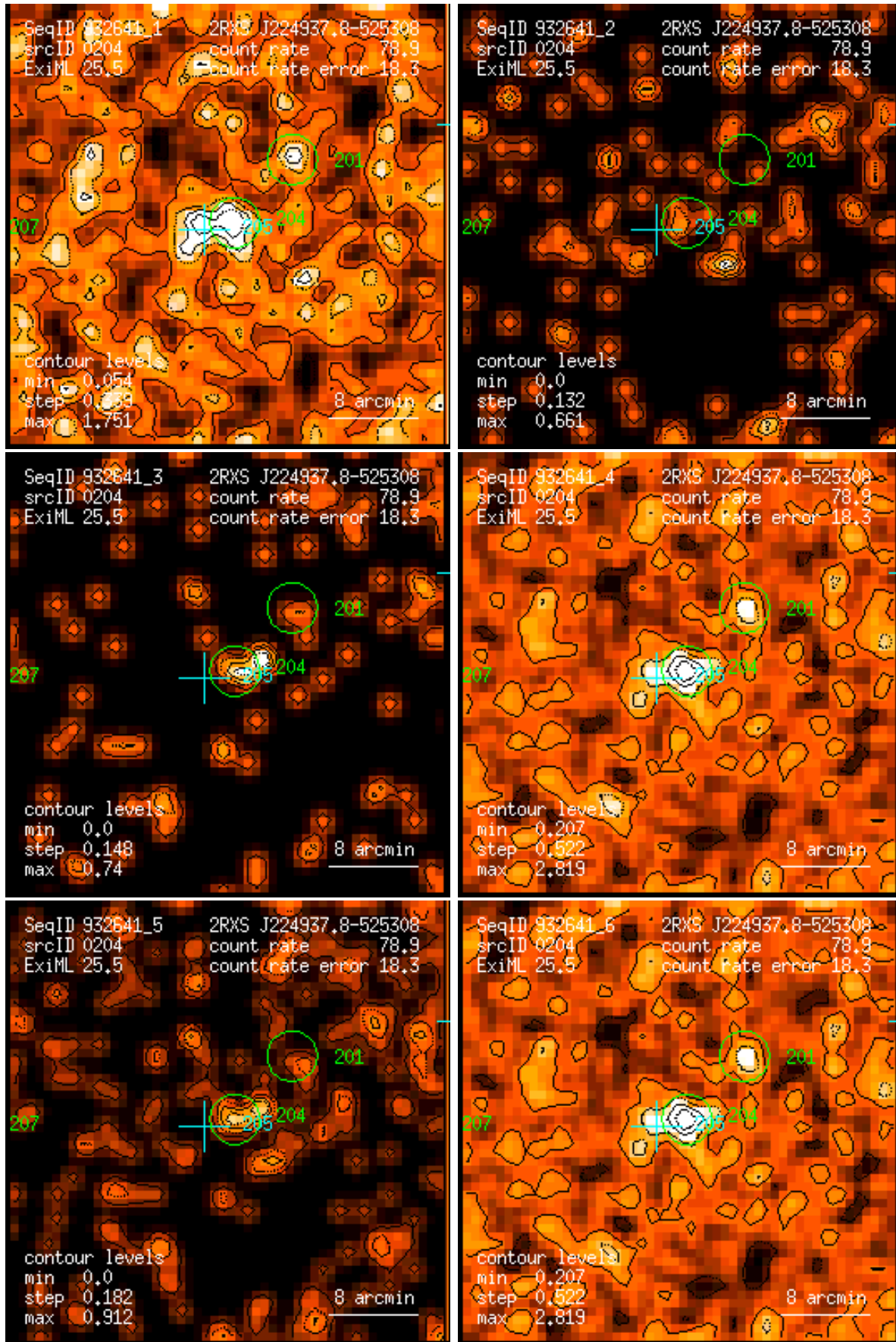
Figure 204: RASS 932641: detection 0204: band rate images, Gaussian filter: (1) PSPC channels 11 – 41, (2) 52 – 90, (3) 91 – 201, (4) 11 – 235, (5) 52 – 201, (6) 11 – 201. Broad band rates in counts/ks. Band rate contour levels in counts/ks/arcmin 2 .
