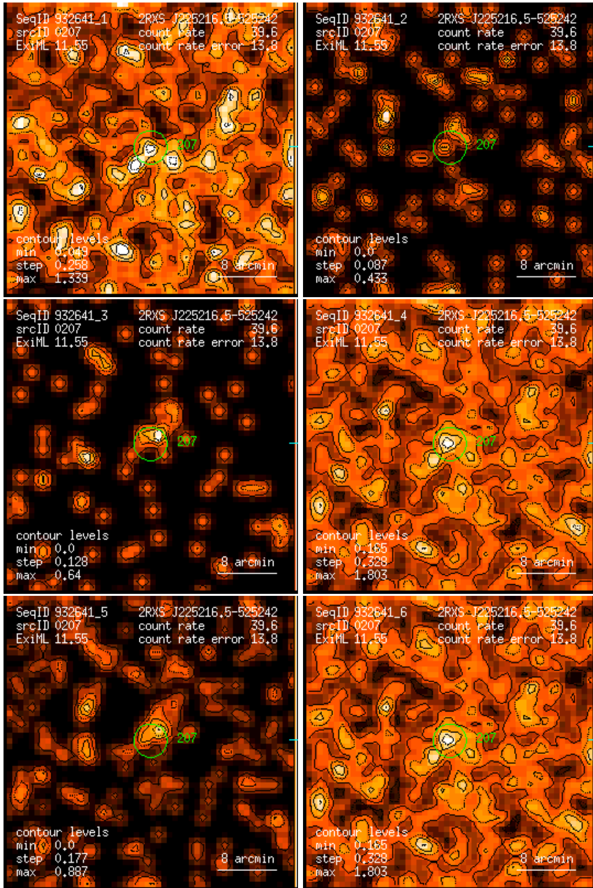
Figure 207: RASS 932641: detection 0207: band rate images, Gaussian filter: (1) PSPC channels 11 – 41, (2) 52 – 90, (3) 91 – 201, (4) 11 – 235, (5) 52 – 201, (6) 11 – 201. Broad band rates in counts/ks. Band rate contour levels in counts/ks/arcmin 2 .
