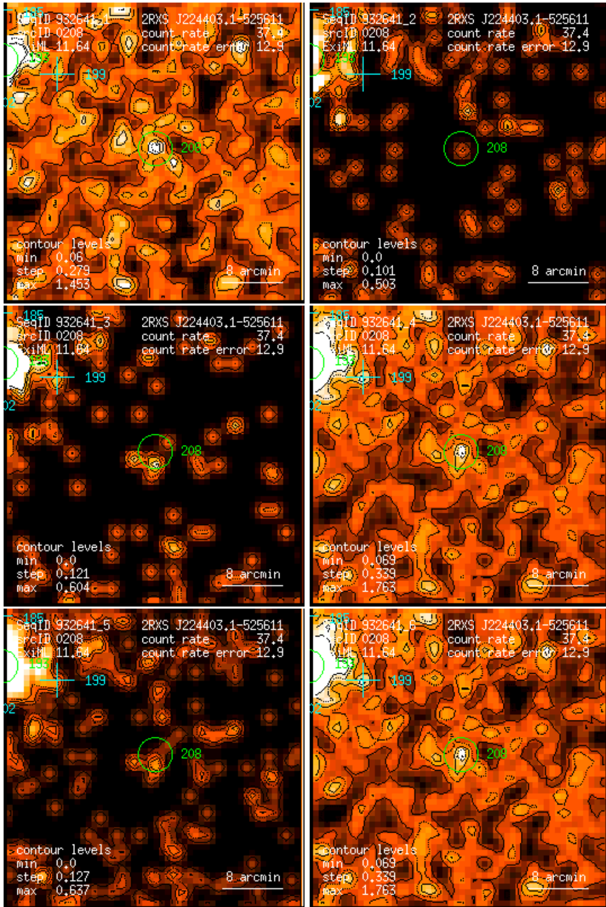
Figure 208: RASS 932641: detection 0208: band rate images, Gaussian filter: (1) PSPC channels 11 – 41, (2) 52 – 90, (3) 91 – 201, (4) 11 – 235, (5) 52 – 201, (6) 11 – 201. Broad band rates in counts/ks. Band rate contour levels in counts/ks/arcmin 2 .
