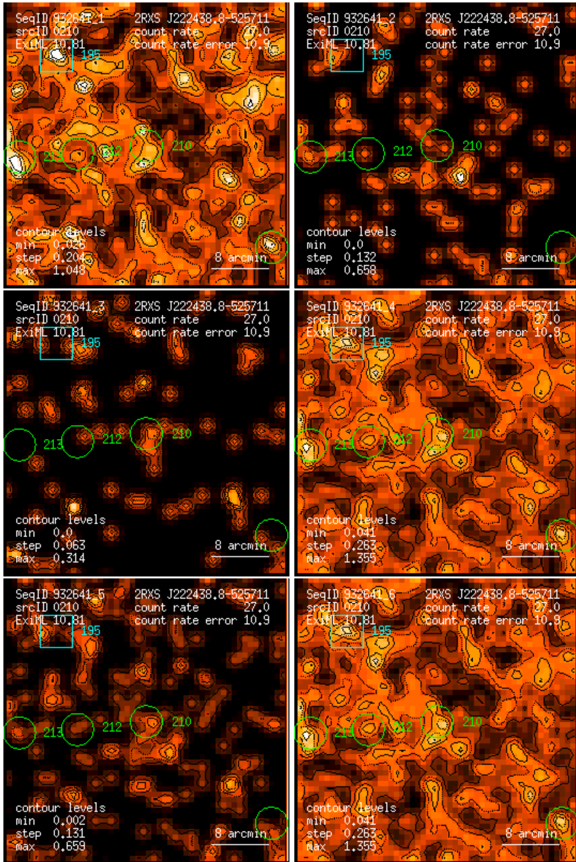
Figure 210: RASS 932641: detection 0210: band rate images, Gaussian filter: (1) PSPC channels 11 – 41, (2) 52 – 90, (3) 91 – 201, (4) 11 – 235, (5) 52 – 201, (6) 11 – 201. Broad band rates in counts/ks. Band rate contour levels in counts/ks/arcmin 2 .
