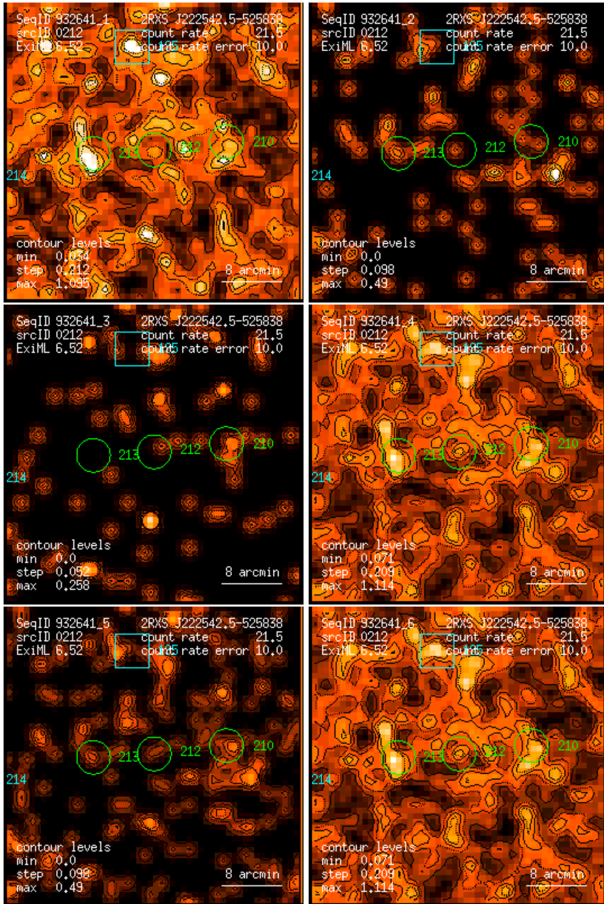
Figure 212: RASS 932641: detection 0212: band rate images, Gaussian filter: (1) PSPC channels 11 – 41, (2) 52 – 90, (3) 91 – 201, (4) 11 – 235, (5) 52 – 201, (6) 11 – 201. Broad band rates in counts/ks. Band rate contour levels in counts/ks/arcmin 2 .
