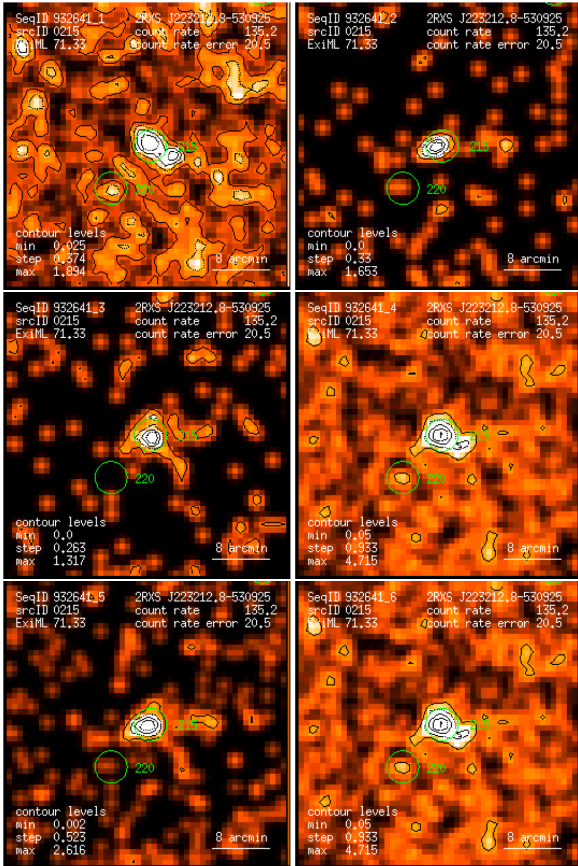
Figure 215: RASS 932641: detection 0215: band rate images, Gaussian filter: (1) PSPC channels 11 – 41, (2) 52 – 90, (3) 91 – 201, (4) 11 – 235, (5) 52 – 201, (6) 11 – 201. Broad band rates in counts/ks. Band rate contour levels in counts/ks/arcmin 2 .
