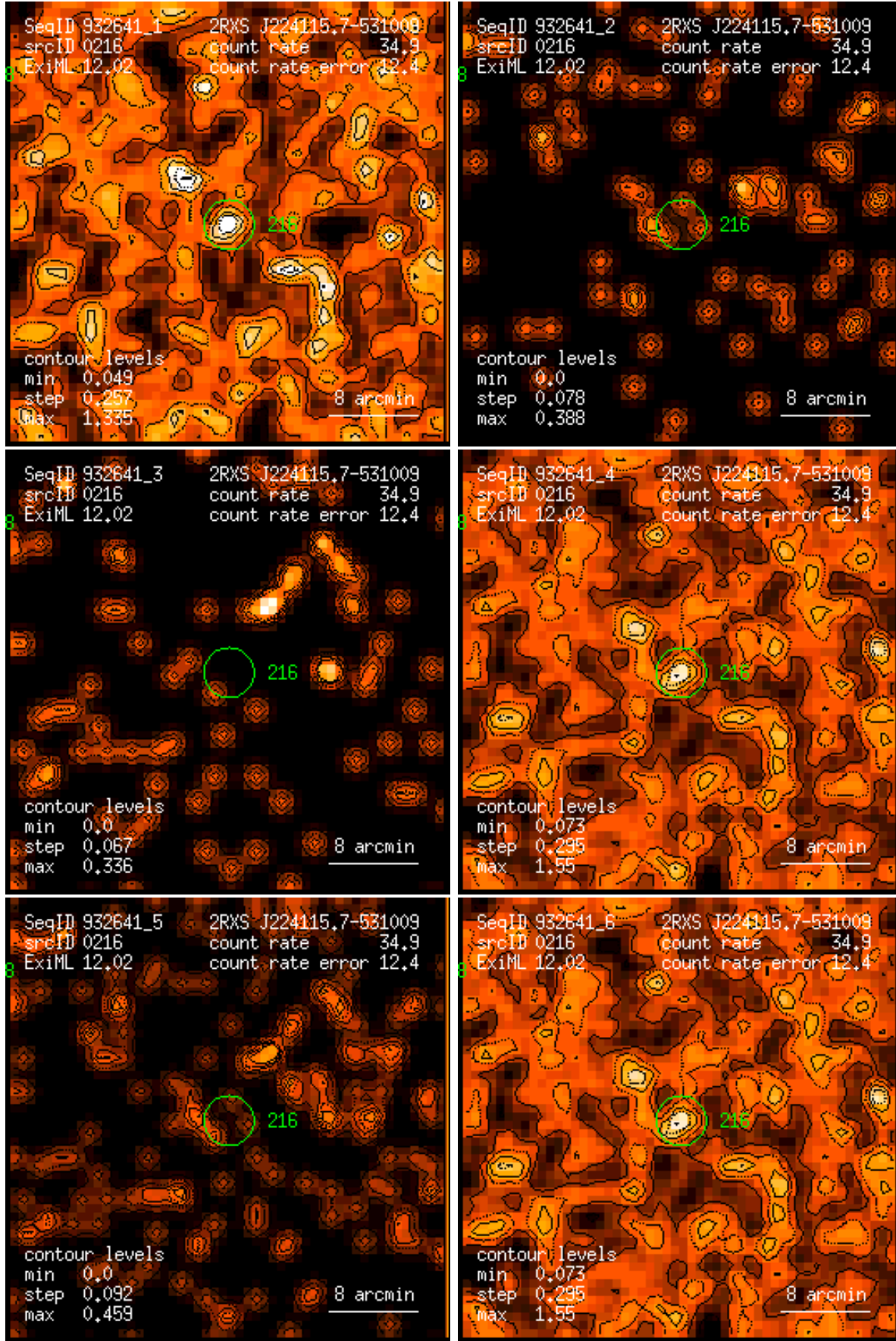
Figure 216: RASS 932641: detection 0216: band rate images, Gaussian filter: (1) PSPC channels 11 – 41, (2) 52 – 90, (3) 91 – 201, (4) 11 – 235, (5) 52 – 201, (6) 11 – 201. Broad band rates in counts/ks. Band rate contour levels in counts/ks/arcmin 2 .
