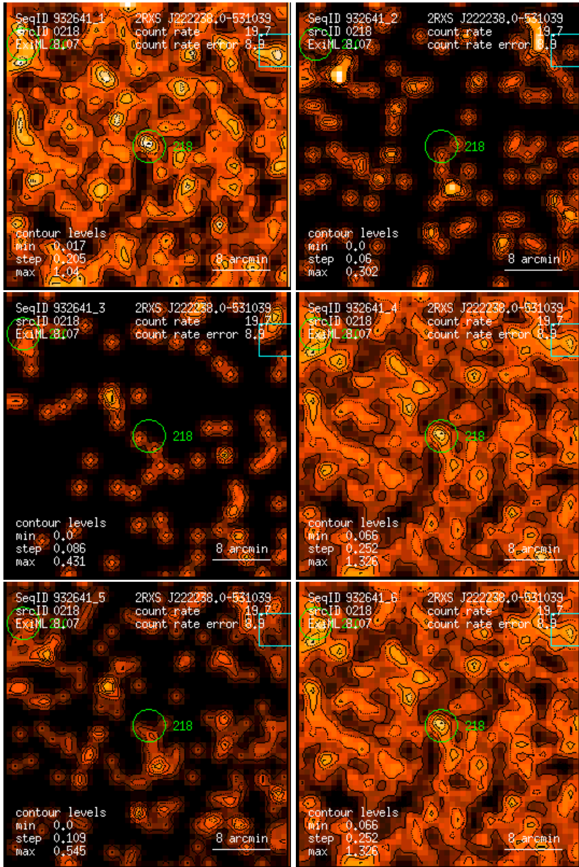
Figure 218: RASS 932641: detection 0218: band rate images, Gaussian filter: (1) PSPC channels 11 – 41, (2) 52 – 90, (3) 91 – 201, (4) 11 – 235, (5) 52 – 201, (6) 11 – 201. Broad band rates in counts/ks. Band rate contour levels in counts/ks/arcmin 2 .
