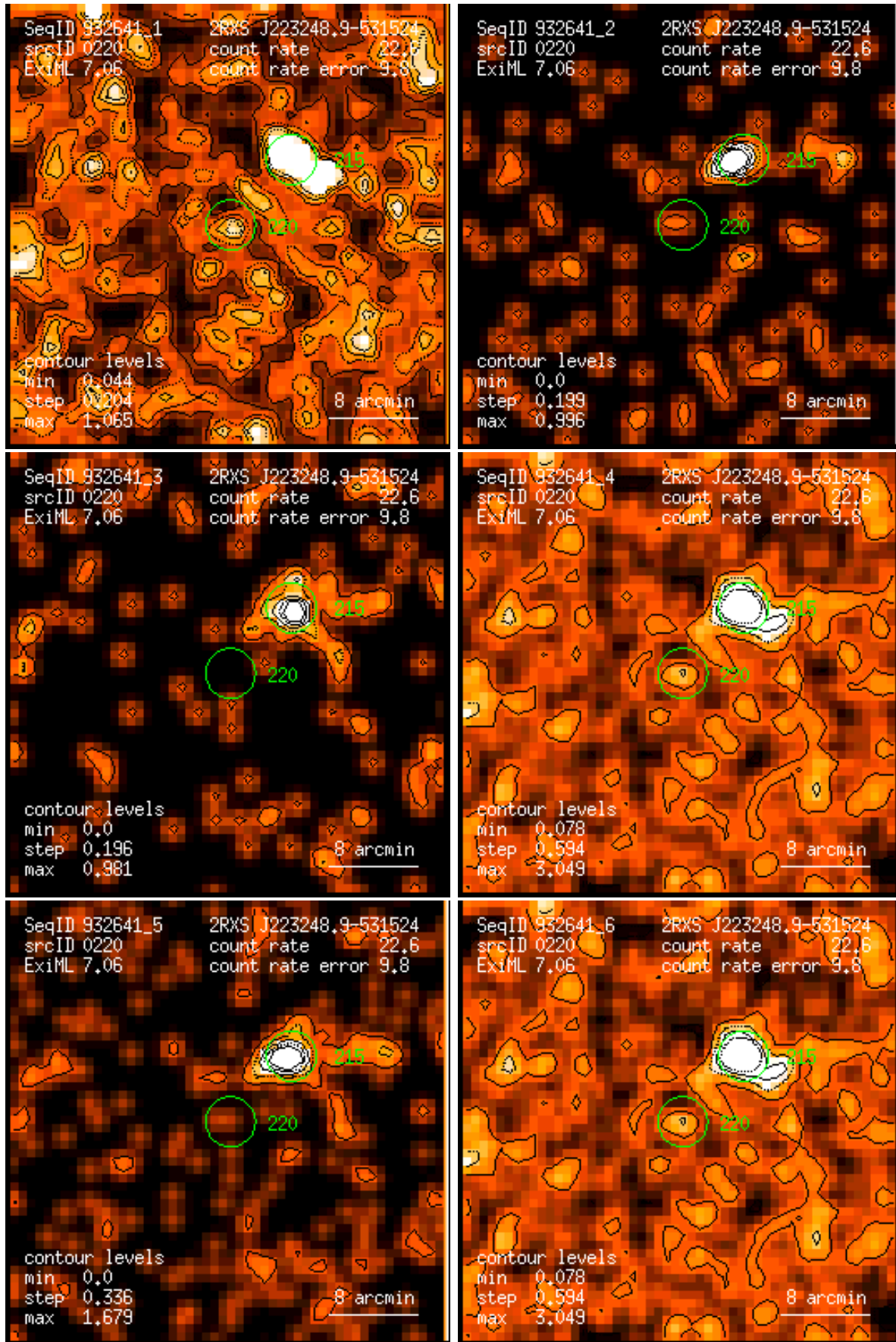
Figure 220: RASS 932641: detection 0220: band rate images, Gaussian filter: (1) PSPC channels 11 – 41, (2) 52 – 90, (3) 91 – 201, (4) 11 – 235, (5) 52 – 201, (6) 11 – 201. Broad band rates in counts/ks. Band rate contour levels in counts/ks/arcmin 2 .
