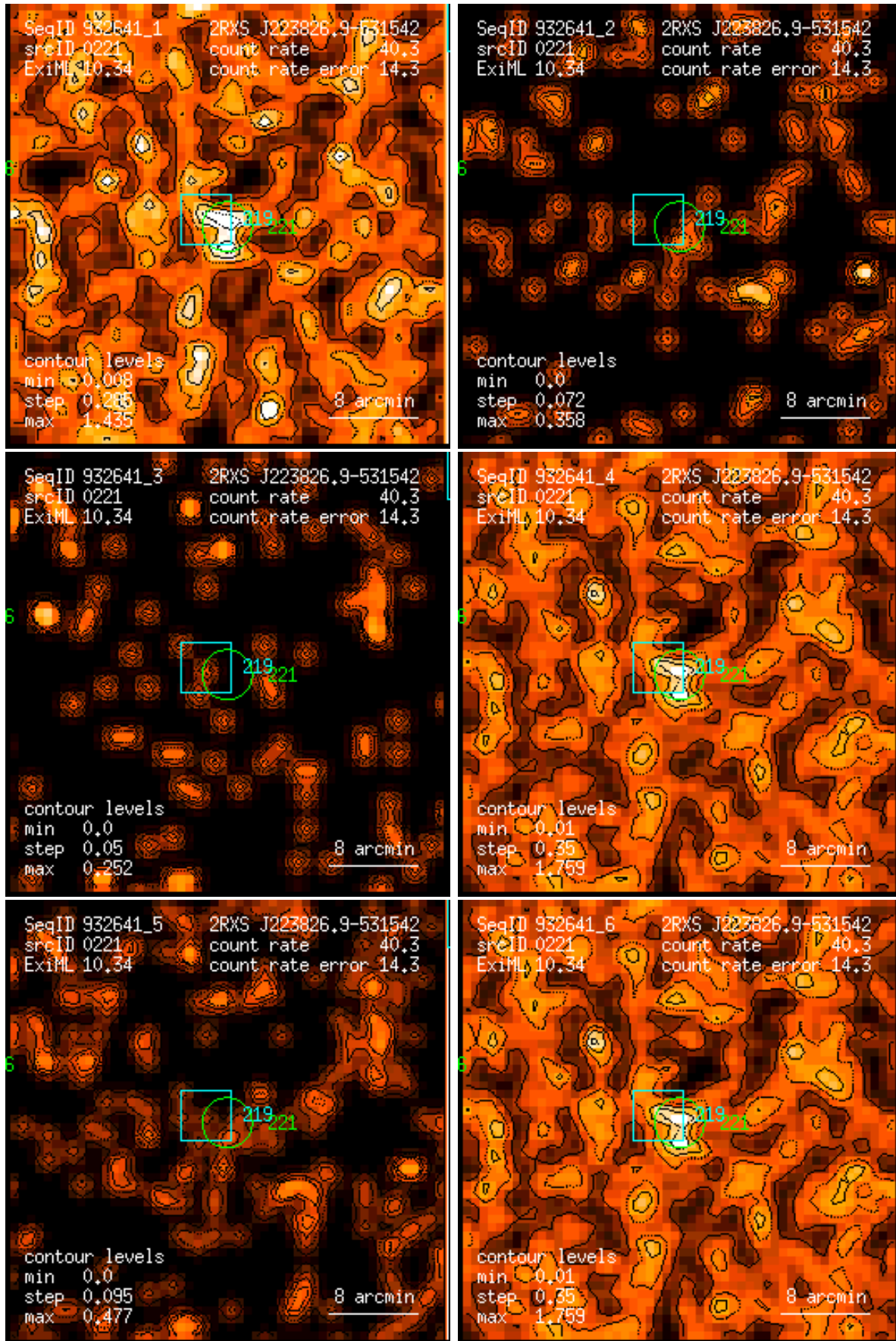
Figure 221: RASS 932641: detection 0221: band rate images, Gaussian filter: (1) PSPC channels 11 – 41, (2) 52 – 90, (3) 91 – 201, (4) 11 – 235, (5) 52 – 201, (6) 11 – 201. Broad band rates in counts/ks. Band rate contour levels in counts/ks/arcmin 2 .
