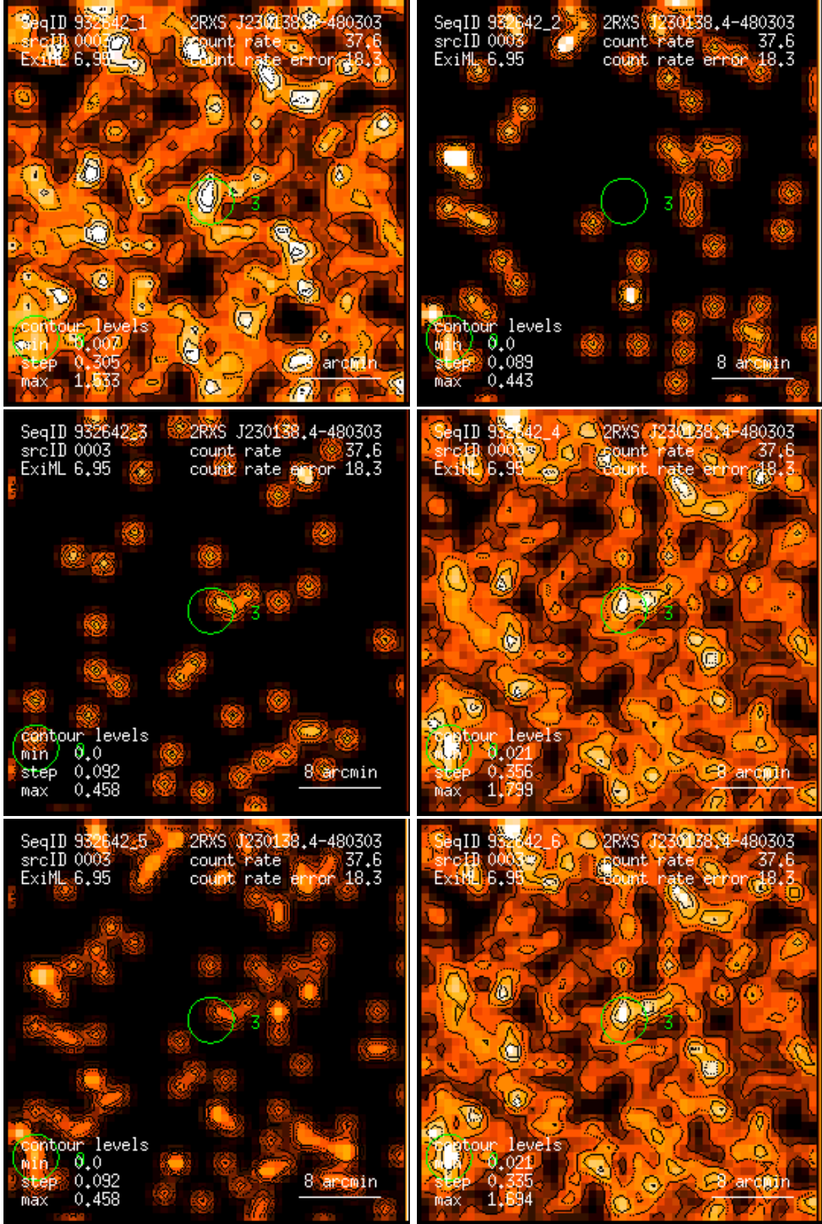
Figure 3: RASS 932642: detection 0003: band rate images, Gaussian filter: (1) PSPC channels 11 – 41, (2) 52 – 90, (3) 91 – 201, (4) 11 – 235, (5) 52 – 201, (6) 11 – 201. Broad band rates in counts/ks. Band rate contour levels in counts/ks/arcmin 2 .
