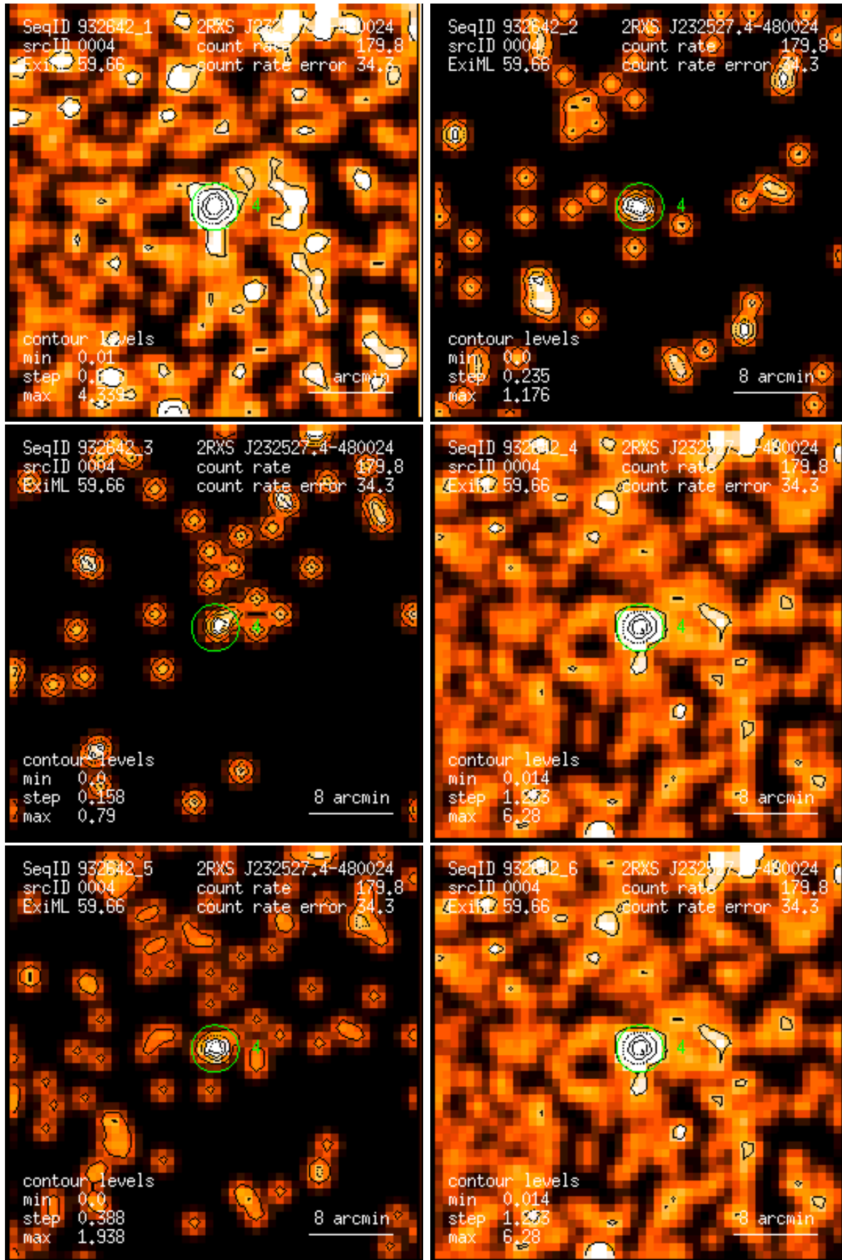
Figure 4: RASS 932642: detection 0004: band rate images, Gaussian filter: (1) PSPC channels 11 – 41, (2) 52 – 90, (3) 91 – 201, (4) 11 – 235, (5) 52 – 201, (6) 11 – 201. Broad band rates in counts/ks. Band rate contour levels in counts/ks/arcmin 2 .
