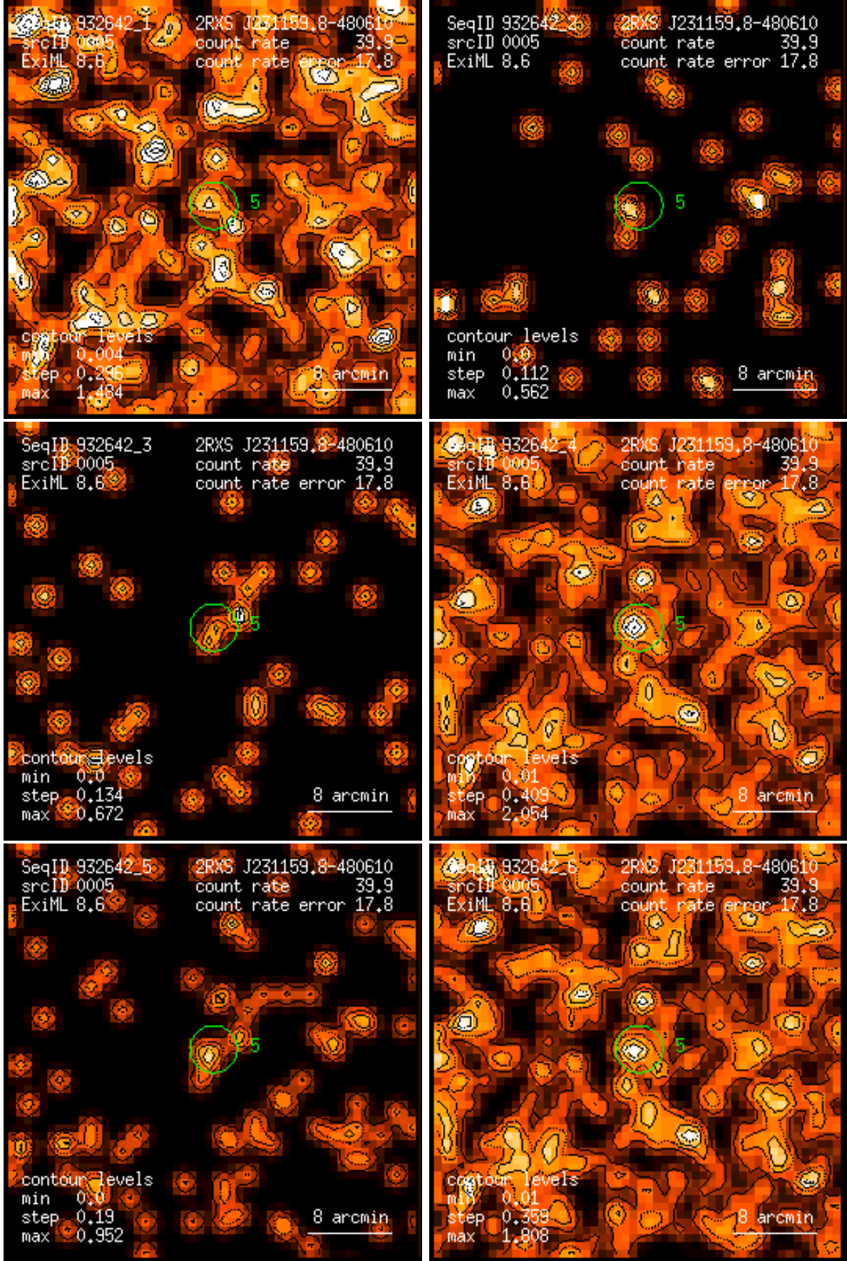
Figure 5: RASS 932642: detection 0005: band rate images, Gaussian filter: (1) PSPC channels 11 – 41, (2) 52 – 90, (3) 91 – 201, (4) 11 – 235, (5) 52 – 201, (6) 11 – 201. Broad band rates in counts/ks. Band rate contour levels in counts/ks/arcmin 2 .
