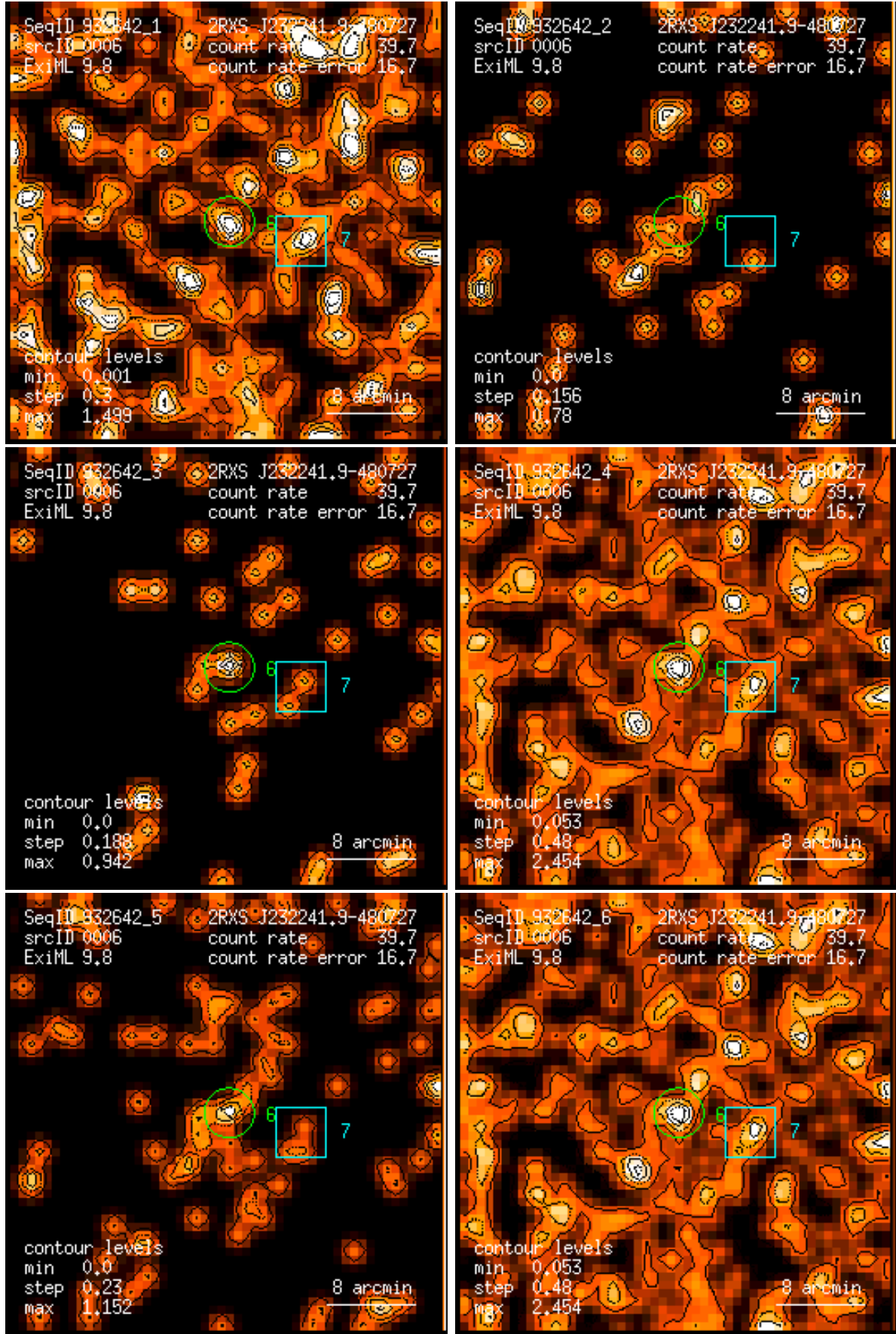
Figure 6: RASS 932642: detection 0006: band rate images, Gaussian filter: (1) PSPC channels 11 – 41, (2) 52 – 90, (3) 91 – 201, (4) 11 – 235, (5) 52 – 201, (6) 11 – 201. Broad band rates in counts/ks. Band rate contour levels in counts/ks/arcmin 2 .
