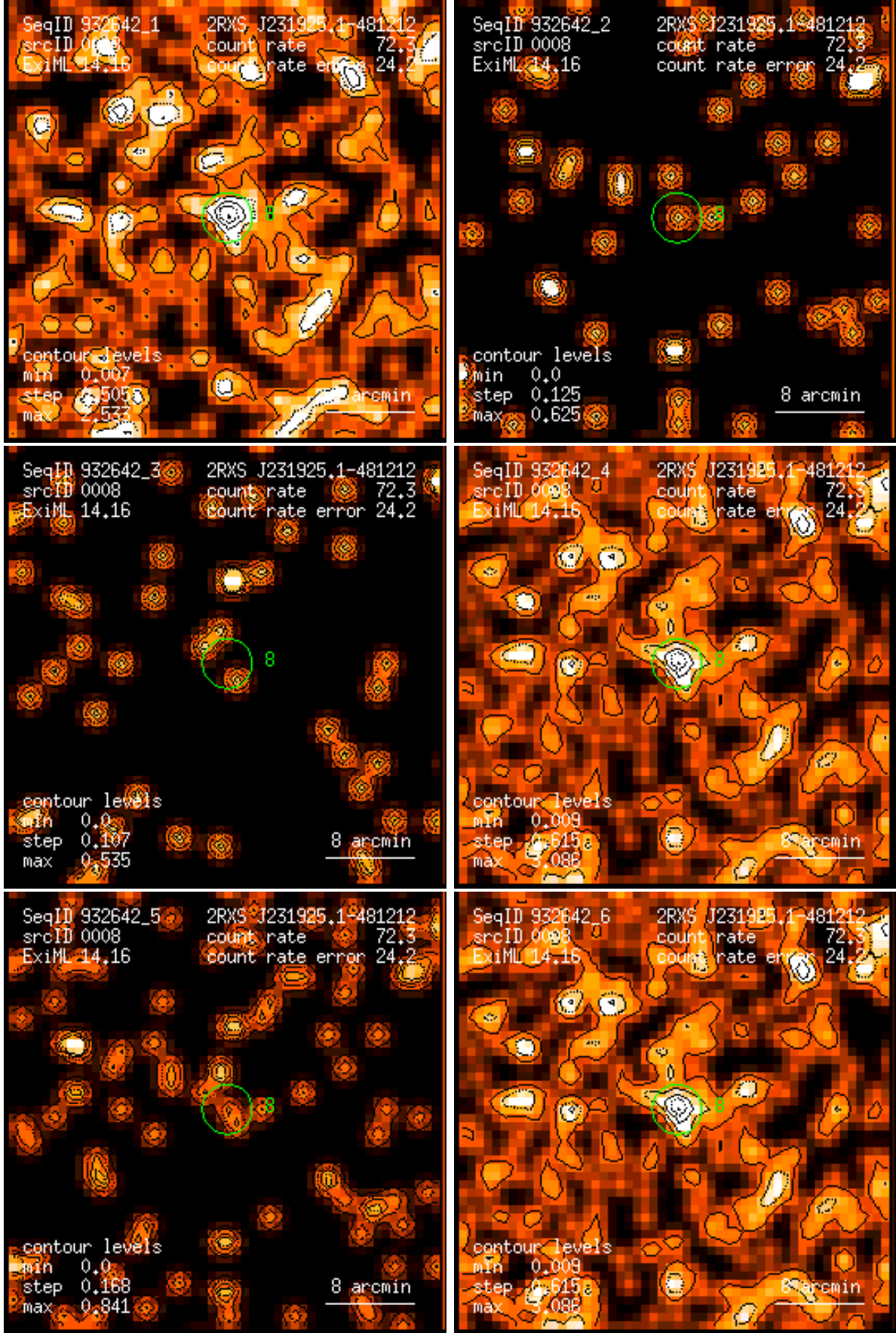
Figure 8: RASS 932642: detection 0008: band rate images, Gaussian filter: (1) PSPC channels 11 – 41, (2) 52 – 90, (3) 91 – 201, (4) 11 – 235, (5) 52 – 201, (6) 11 – 201. Broad band rates in counts/ks. Band rate contour levels in counts/ks/arcmin 2 .
