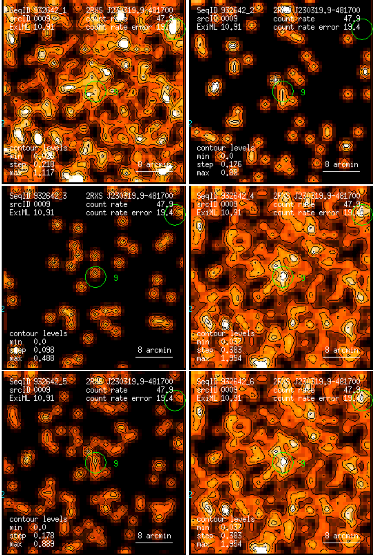
Figure 9: RASS 932642: detection 0009: band rate images, Gaussian filter: (1) PSPC channels 11 – 41, (2) 52 – 90, (3) 91 – 201, (4) 11 – 235, (5) 52 – 201, (6) 11 – 201. Broad band rates in counts/ks. Band rate contour levels in counts/ks/arcmin 2 .
