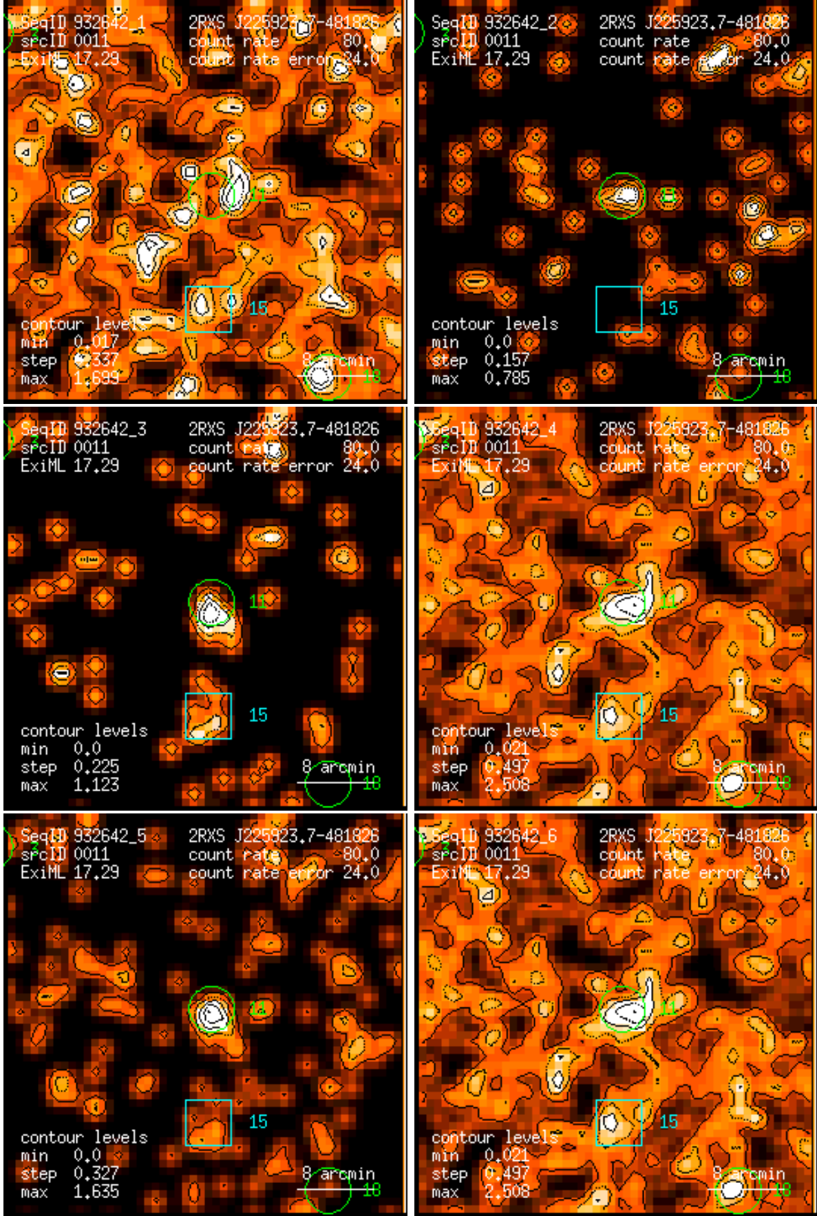
Figure 11: RASS 932642: detection 0011: band rate images, Gaussian filter: (1) PSPC channels 11 – 41, (2) 52 – 90, (3) 91 – 201, (4) 11 – 235, (5) 52 – 201, (6) 11 – 201. Broad band rates in counts/ks. Band rate contour levels in counts/ks/arcmin 2 .
