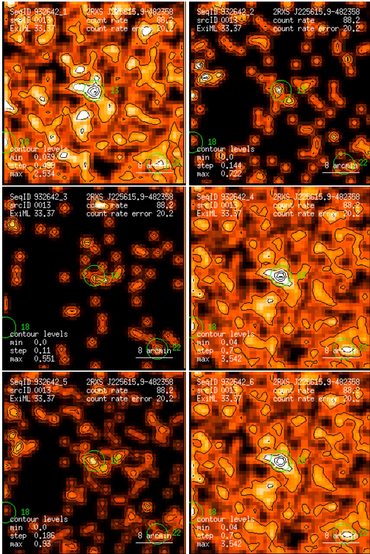
Figure 13: RASS 932642: detection 0013: band rate images, Gaussian filter: (1) PSPC channels 11 – 41, (2) 52 – 90, (3) 91 – 201, (4) 11 – 235, (5) 52 – 201, (6) 11 – 201. Broad band rates in counts/ks. Band rate contour levels in counts/ks/arcmin 2 .
