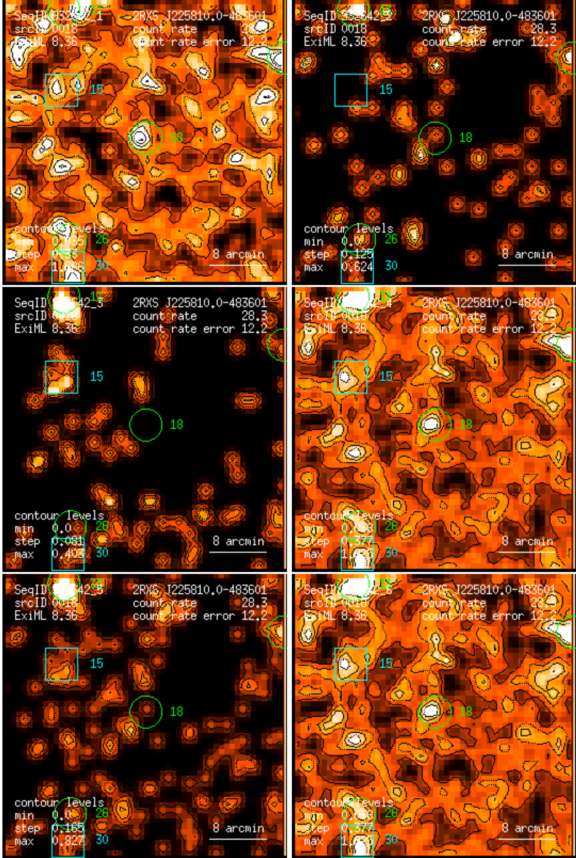
Figure 18: RASS 932642: detection 0018: band rate images, Gaussian filter: (1) PSPC channels 11 – 41, (2) 52 – 90, (3) 91 – 201, (4) 11 – 235, (5) 52 – 201, (6) 11 – 201. Broad band rates in counts/ks. Band rate contour levels in counts/ks/arcmin 2 .
