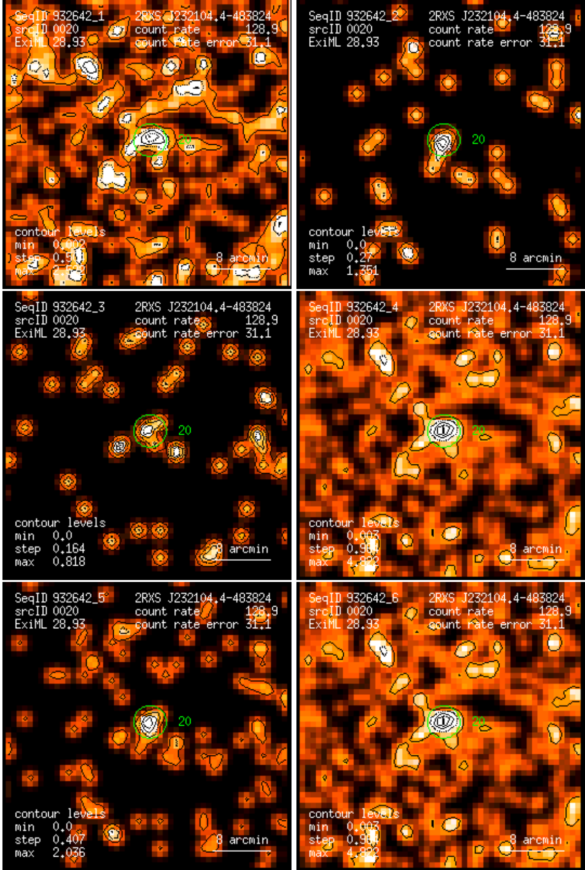
Figure 20: RASS 932642: detection 0020: band rate images, Gaussian filter: (1) PSPC channels 11 – 41, (2) 52 – 90, (3) 91 – 201, (4) 11 – 235, (5) 52 – 201, (6) 11 – 201. Broad band rates in counts/ks. Band rate contour levels in counts/ks/arcmin 2 .
