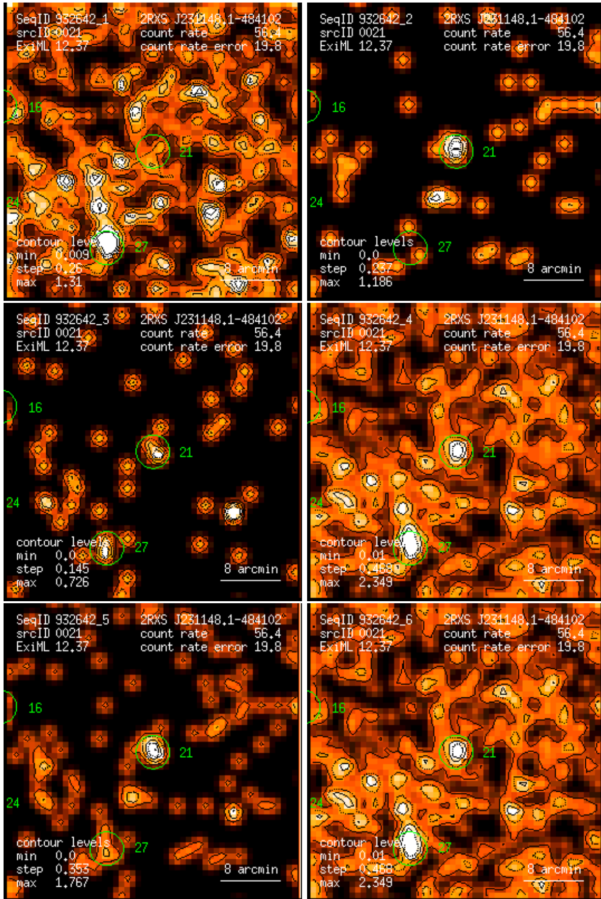
Figure 21: RASS 932642: detection 0021: band rate images, Gaussian filter: (1) PSPC channels 11 – 41, (2) 52 – 90, (3) 91 – 201, (4) 11 – 235, (5) 52 – 201, (6) 11 – 201. Broad band rates in counts/ks. Band rate contour levels in counts/ks/arcmin 2 .
