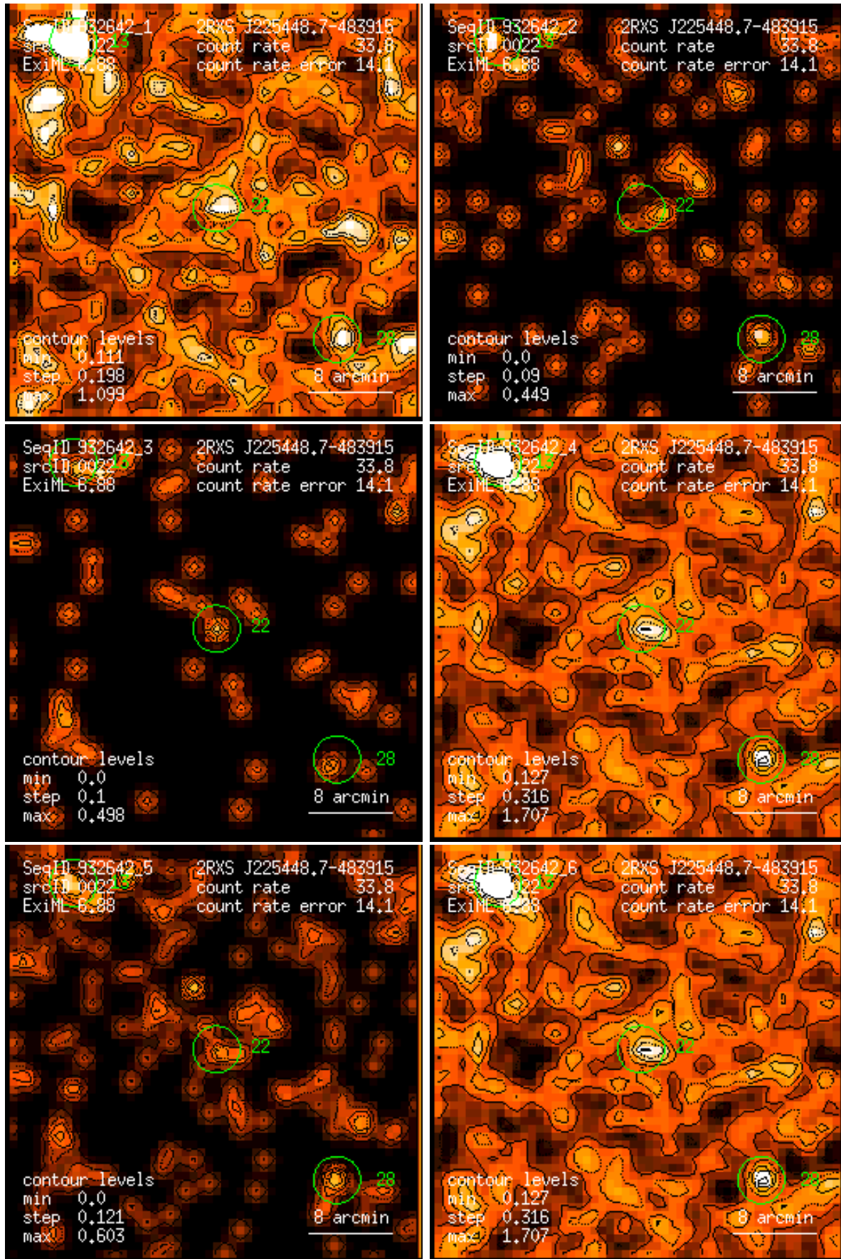
Figure 22: RASS 932642: detection 0022: band rate images, Gaussian filter: (1) PSPC channels 11 – 41, (2) 52 – 90, (3) 91 – 201, (4) 11 – 235, (5) 52 – 201, (6) 11 – 201. Broad band rates in counts/ks. Band rate contour levels in counts/ks/arcmin 2 .
