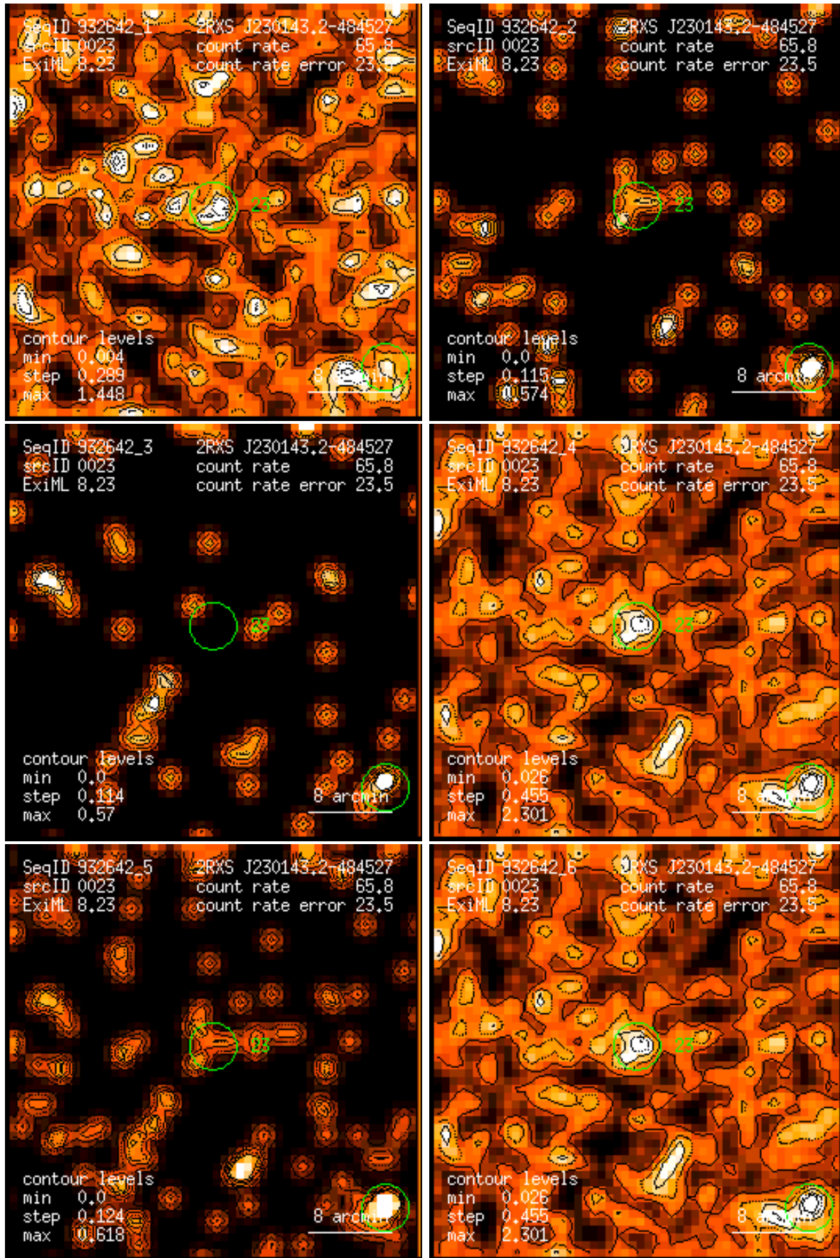
Figure 23: RASS 932642: detection 0023: band rate images, Gaussian filter: (1) PSPC channels 11 – 41, (2) 52 – 90, (3) 91 – 201, (4) 11 – 235, (5) 52 – 201, (6) 11 – 201. Broad band rates in counts/ks. Band rate contour levels in counts/ks/arcmin 2 .
