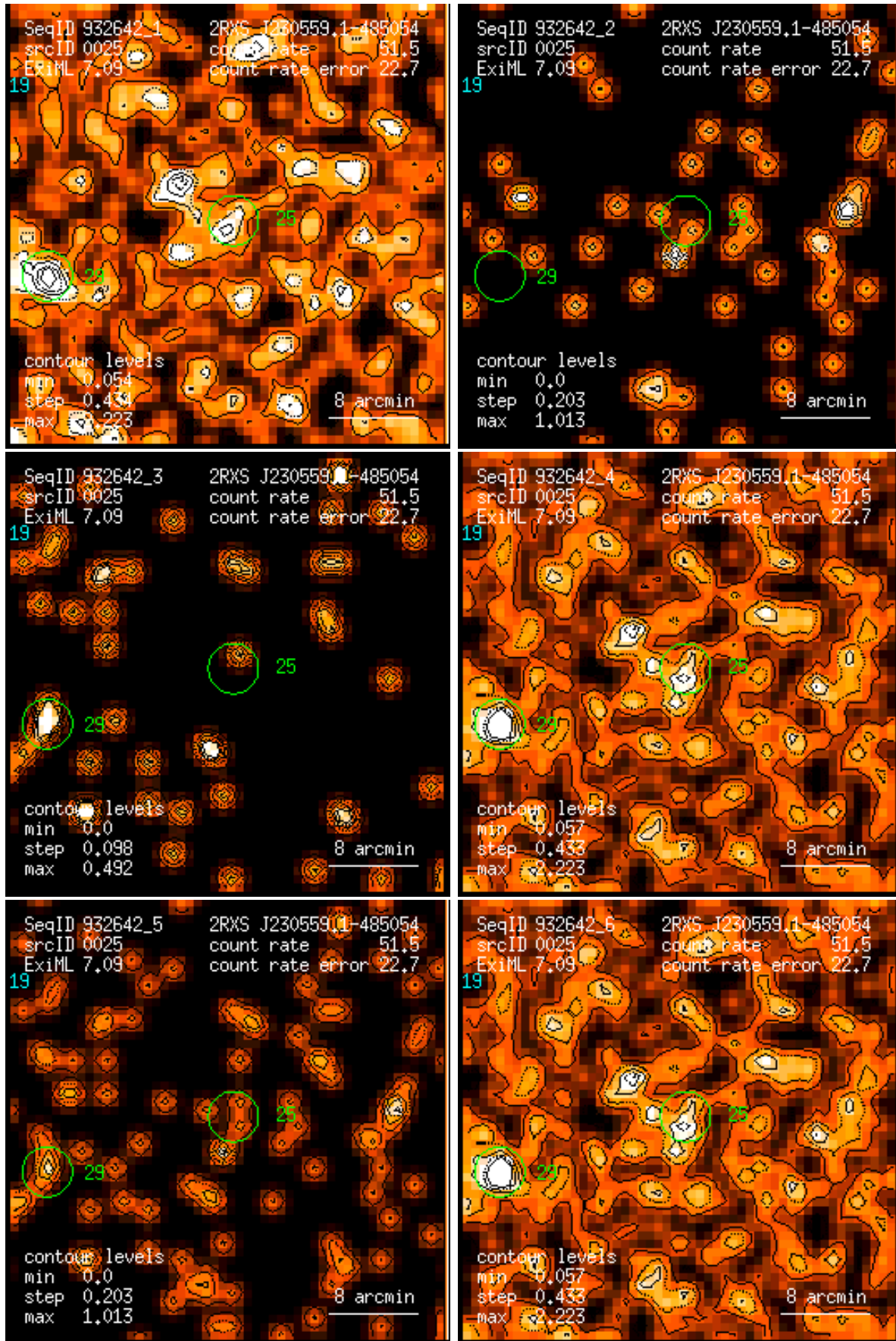
Figure 25: RASS 932642: detection 0025: band rate images, Gaussian filter: (1) PSPC channels 11 – 41, (2) 52 – 90, (3) 91 – 201, (4) 11 – 235, (5) 52 – 201, (6) 11 – 201. Broad band rates in counts/ks. Band rate contour levels in counts/ks/arcmin 2 .
