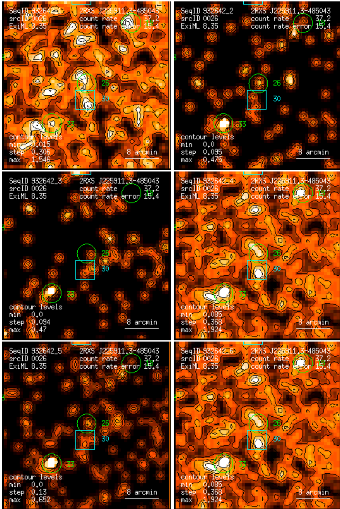
Figure 26: RASS 932642: detection 0026: band rate images, Gaussian filter: (1) PSPC channels 11 – 41, (2) 52 – 90, (3) 91 – 201, (4) 11 – 235, (5) 52 – 201, (6) 11 – 201. Broad band rates in counts/ks. Band rate contour levels in counts/ks/arcmin 2 .
